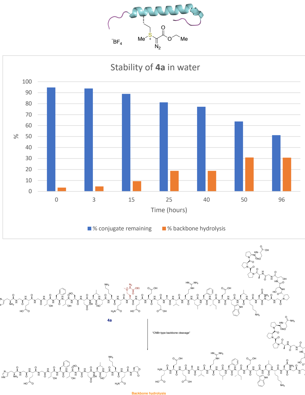
Figure S67: Stability study of 4a in water, over a period of 96 hours, at room temperature. t = 0 hours begins after storage of 4a for 24 hours. Degradation occurs predominantly via backbone hydrolysis.
