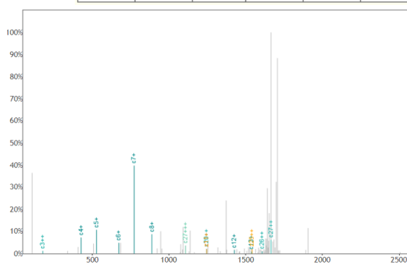
ETD fragmentation spectrum c and z ions
