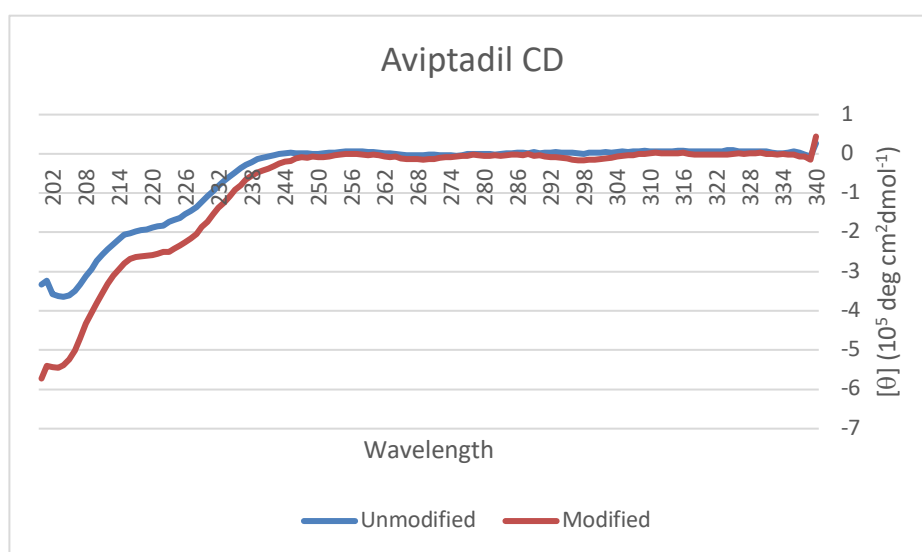
Figure S17. CD spectra of 5 (50 \mu M) in 5 mM pH 7.4 phosphate buffer, and Aviptadil (25 \mu M) in 5 mM pH 7.4 phosphate buffer.
