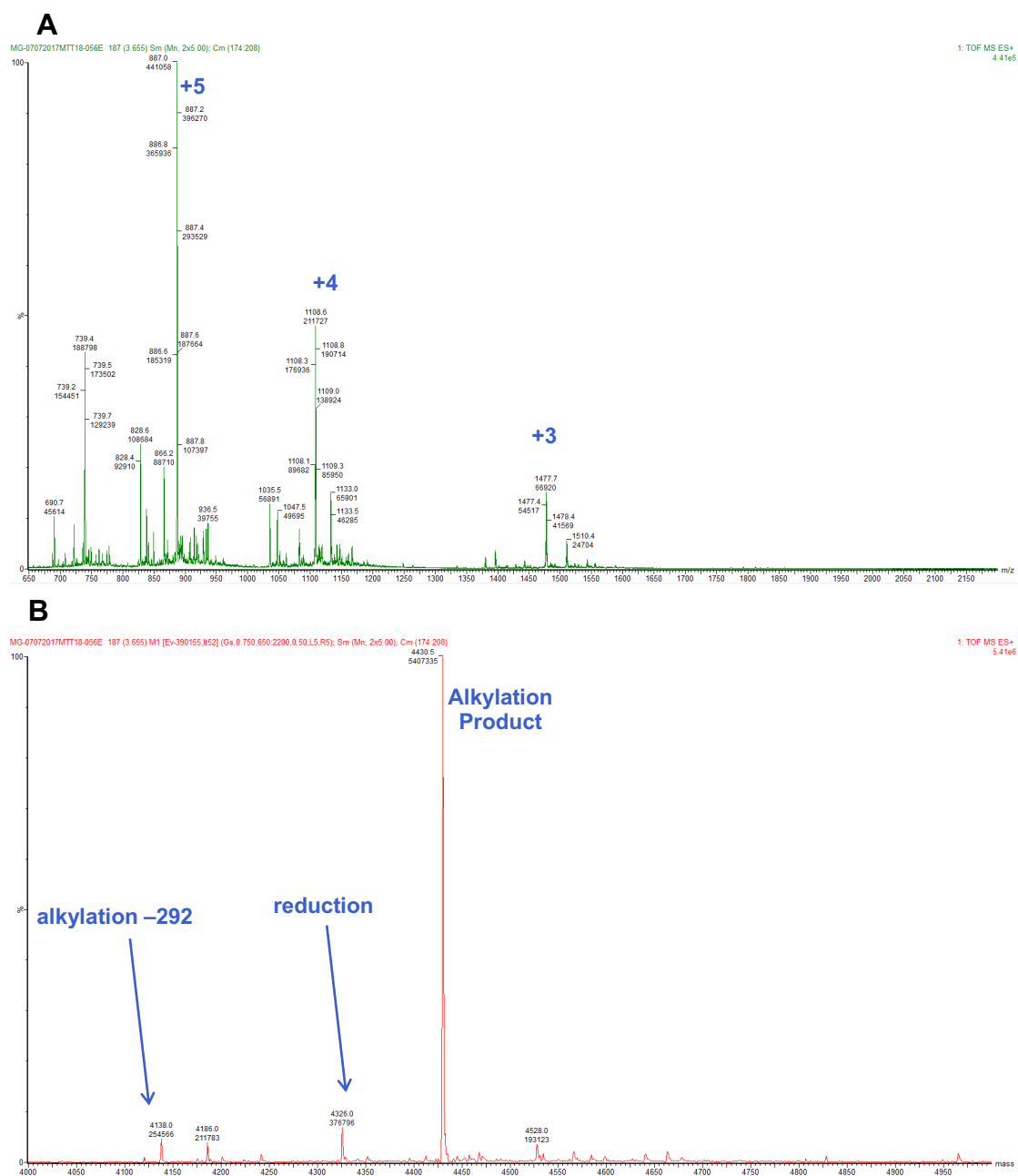
Figure S61. (A) Mass chromatogram of the crude reaction mixture of the photoalkylation of exenatide derivative 4g and Hantzsch ester 14b . (B) Deconvoluted mass chromatogram of the crude reaction mixture.
