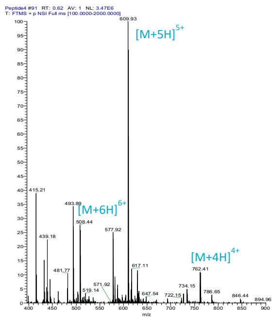
Figure S22: MS Scan of Tetracosactide conjugate 6
