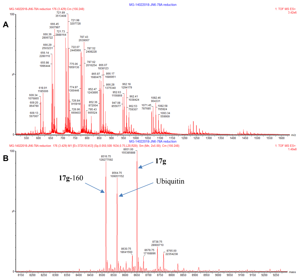
Figure S55: (A) Mass trace of crude two-step reaction of Ubiquitin to form 17g . (B) Deconvoluted mass spectrum of the crude reaction to form 17g .
