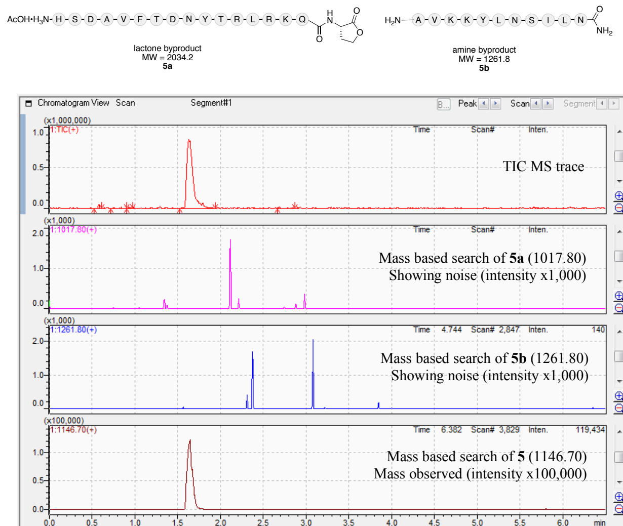
Figure S80: Mass based search on mass trace of crude reaction to form aviptadil conjugate 5 . Search for backbone hydrolysis products (amine byproduct 5b [M+H]^+ = 1261.8 and lactone byproduct 5a [M+2H]^{2+} = 1017.8 ) shows only noise, whilst search for one of the product ions of 5 ( [(M^+) + 2H]^{3+} = 1146.7 ) clearly shows the presence of aviptadil conjugate 5 .
