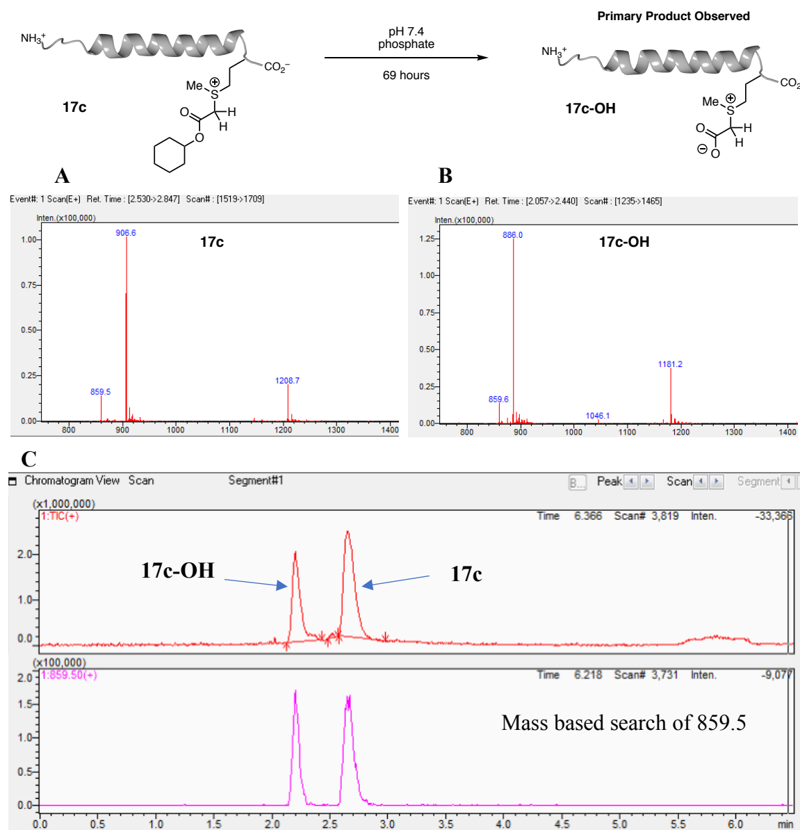
Figure S75: (A) Mass trace of glucagon cyclohexyl conjugate 17c . (B) Mass trace of glucagon hydrolysis product 17c-OH . (C) Mass based search of fragment ion (MW = 859.5), showing the fragment ion is present in both compounds 17c and 17c-OH , both of which elute at different retention times.
