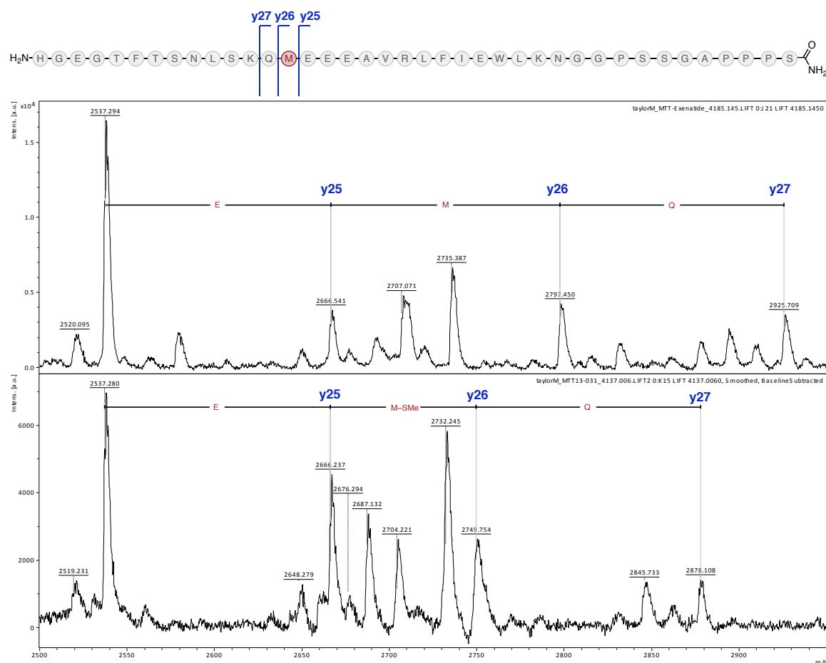
Figure S9. (A) MS/MS chromatogram of Exenatide ( 4 ) highlighting the y25, y26, and y27 fragments. (B) MS/MS chromatogram of conjugate 4f highlighting the y25, y26, and y27 fragments of ( 4f -170) + fragment. The difference of 48 mass units on the y26 mass between the two spectra confirm modification of the methionine residue in exenatide.
