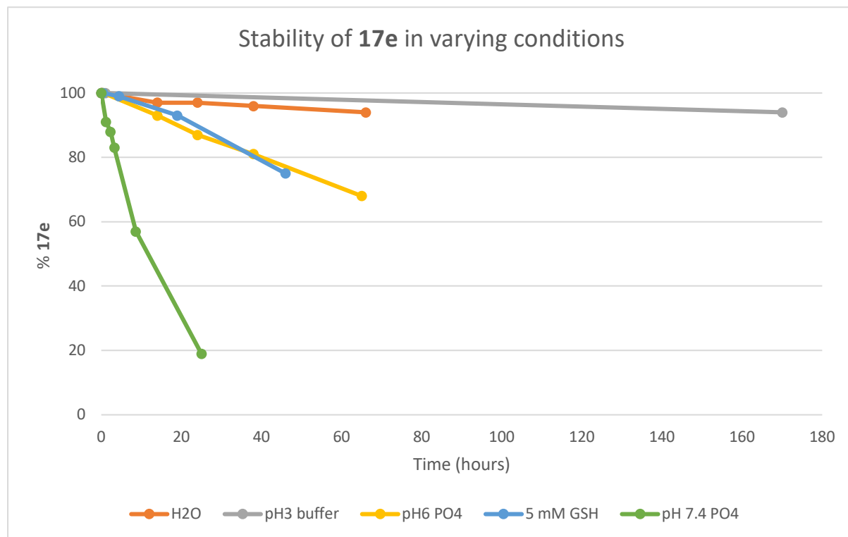
Figure S70: The stability profile of 17e . For each experiment, 17e (100 \mu M) was allowed to stand in solution at room temperature (21°C) over the time course and analyzed by LCMS. In all instances, degradation of 17e occurs via the hydrolysis of the ester moiety to yield a free carboxylate.
