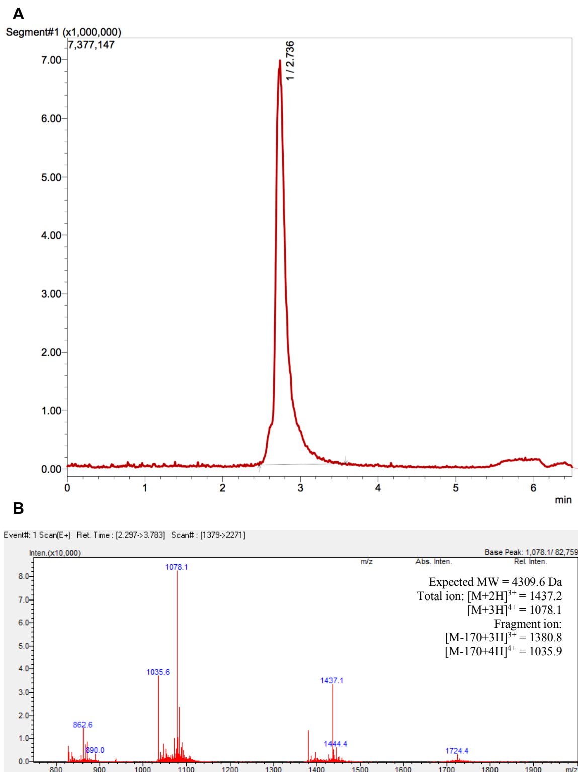
Figure S8. (A) Mass trace of purified 4f. (B) Mass spectrum of purified 4f.
