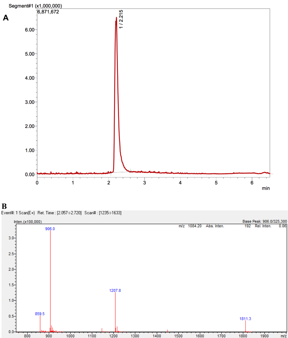
Figure S51. (A) HPLC trace Purified 17e. B) Mass spectrum of purified 17e (TIC from 2.06-2.72 min).
