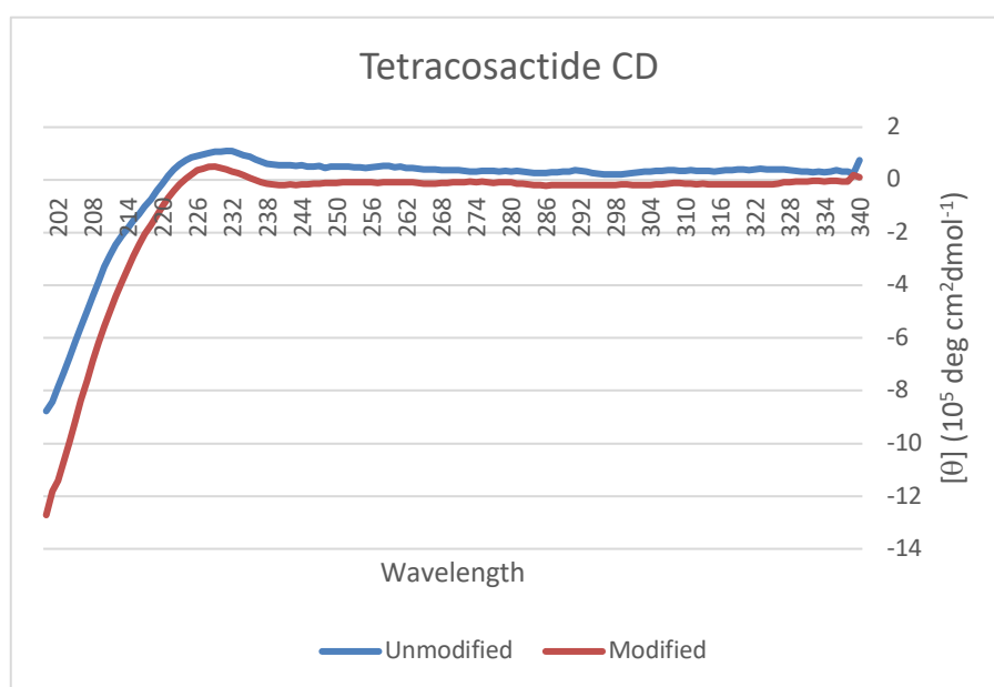
Figure S24. CD spectra of 6 (50 \mu M) in 5 mM pH 7.4 phosphate buffer, and Tetracosactide (25 \mu M) in 5 mM pH 7.4 phosphate buffer
