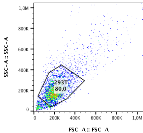
Population Gating
