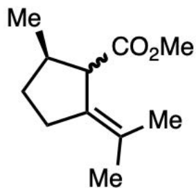
methyl pulegenate (12)
