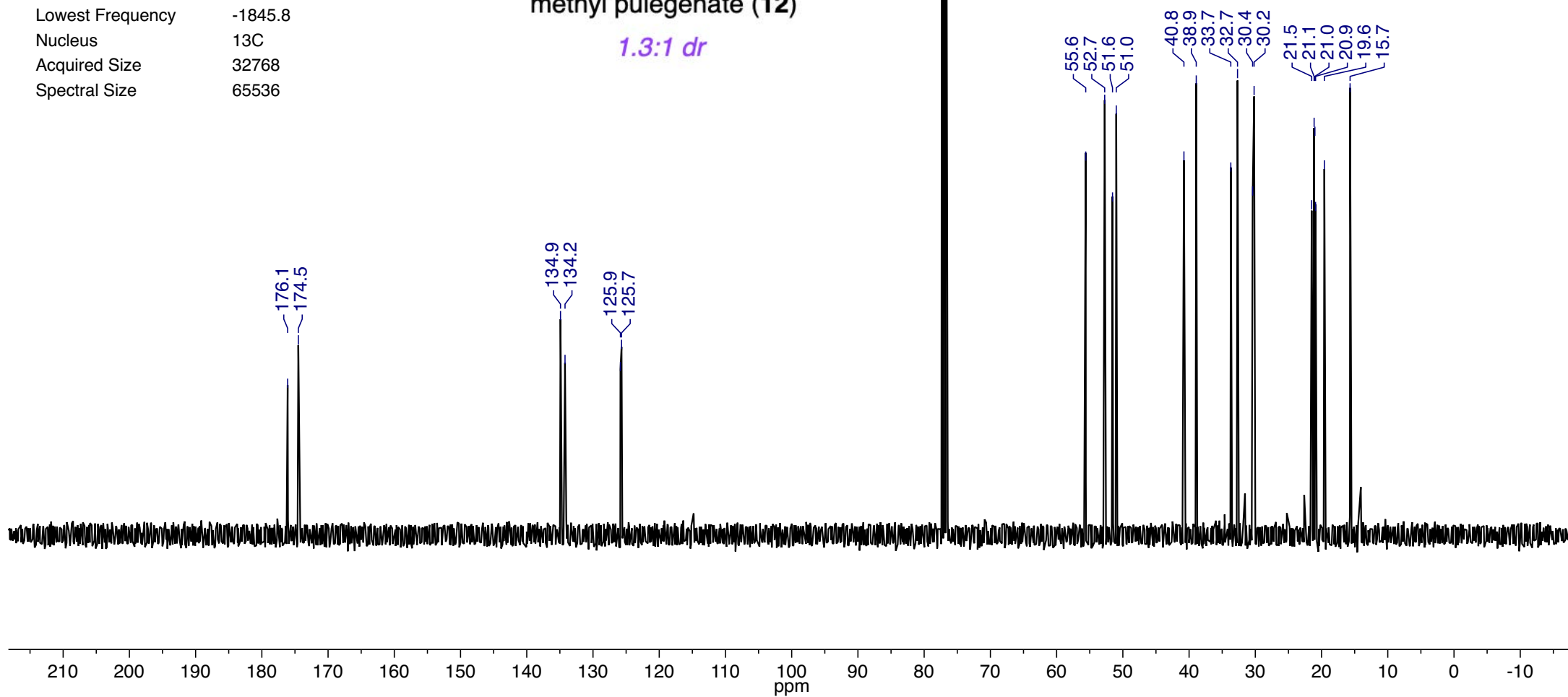
methyl pulegenate (12)
