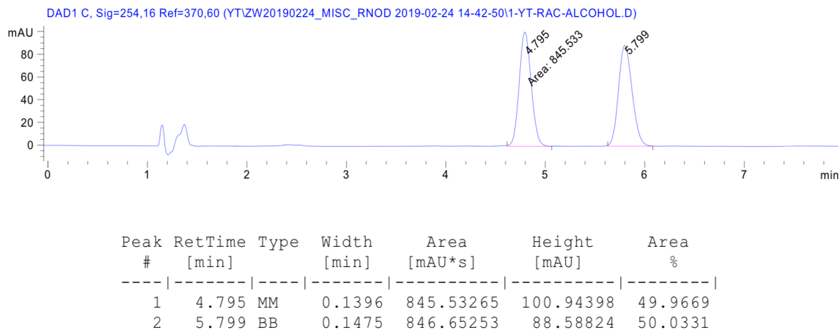
Figure S3. SFC traces of racemic and enantioenriched alcohol 27 .
