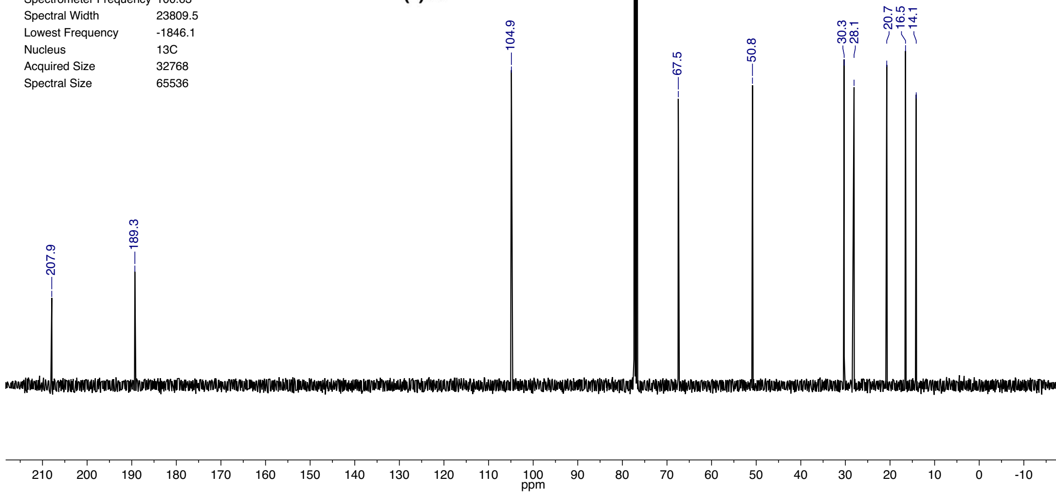
(±)-21
