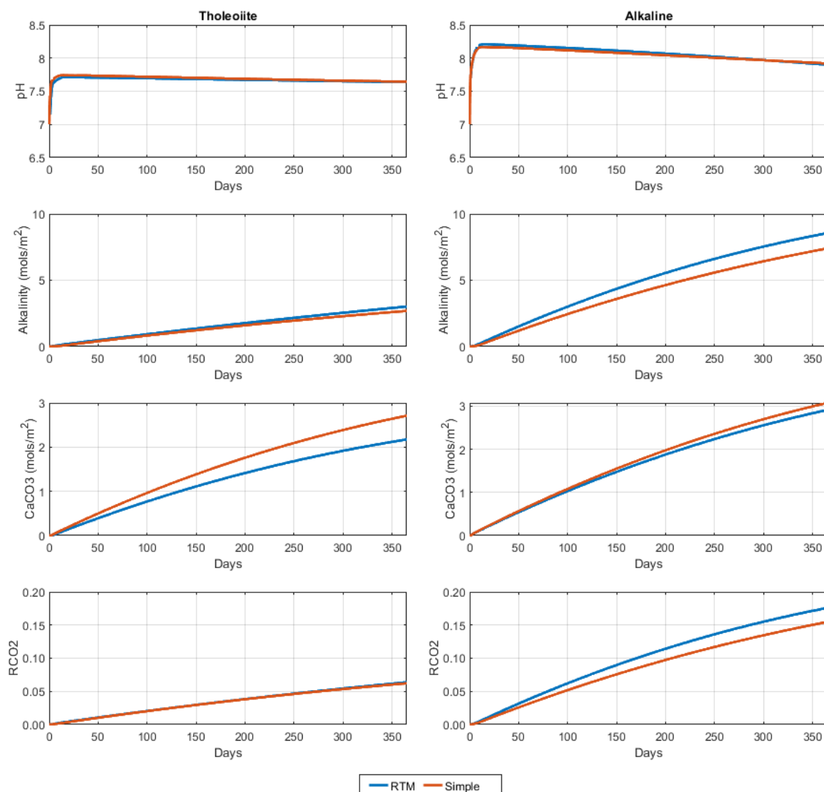
Figure S12 Comparison of pH and carbon removal systems in the RTM and performance model.
