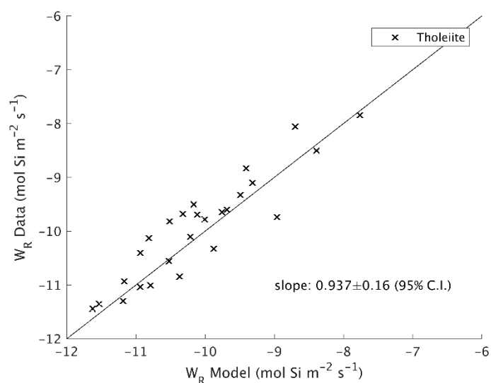
Figure S3. Model validation. Plots show predicted weathering rate ( W_R , \log_{10} scale) with our performance model rate equation (Si-release) validated against observations of flask-based weathering rates, based on an extensive data compilation 14 , for (a) the alkali basalt (fast weathering) and (b) tholeiitic basalt (slow weathering). Weathering rates between the two types of basalt differ by a factor of 2; about 0.3 on the \log_{10} scale of the plots. Slopes are not significantly different from 1 ( F -test, P < 0.001 for both plots).
