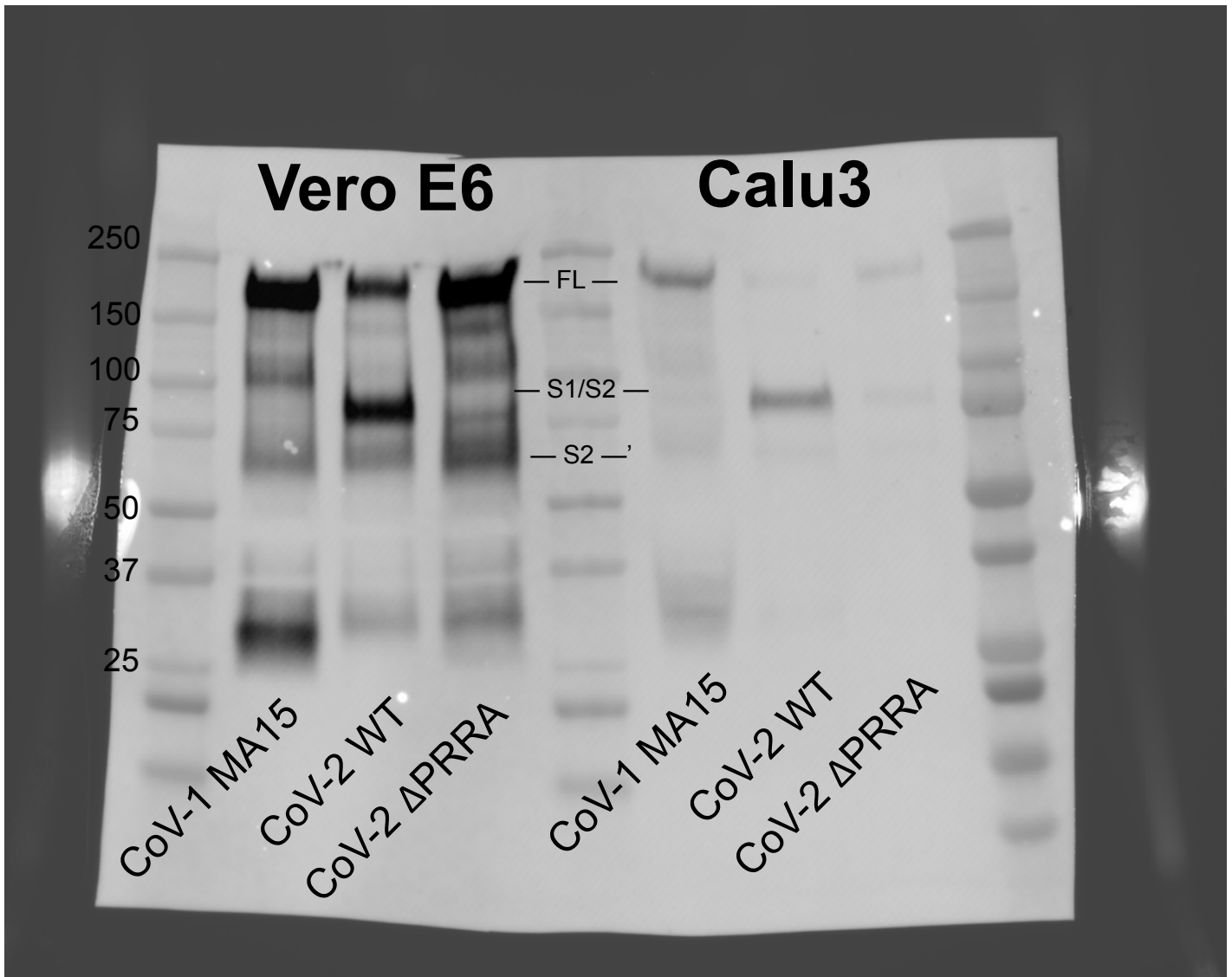
Supplementary Figure 1. Uncropped chemiluminescent images of Western blots for CoV Spike proteins from top panels of Figures 1d and 1g.
