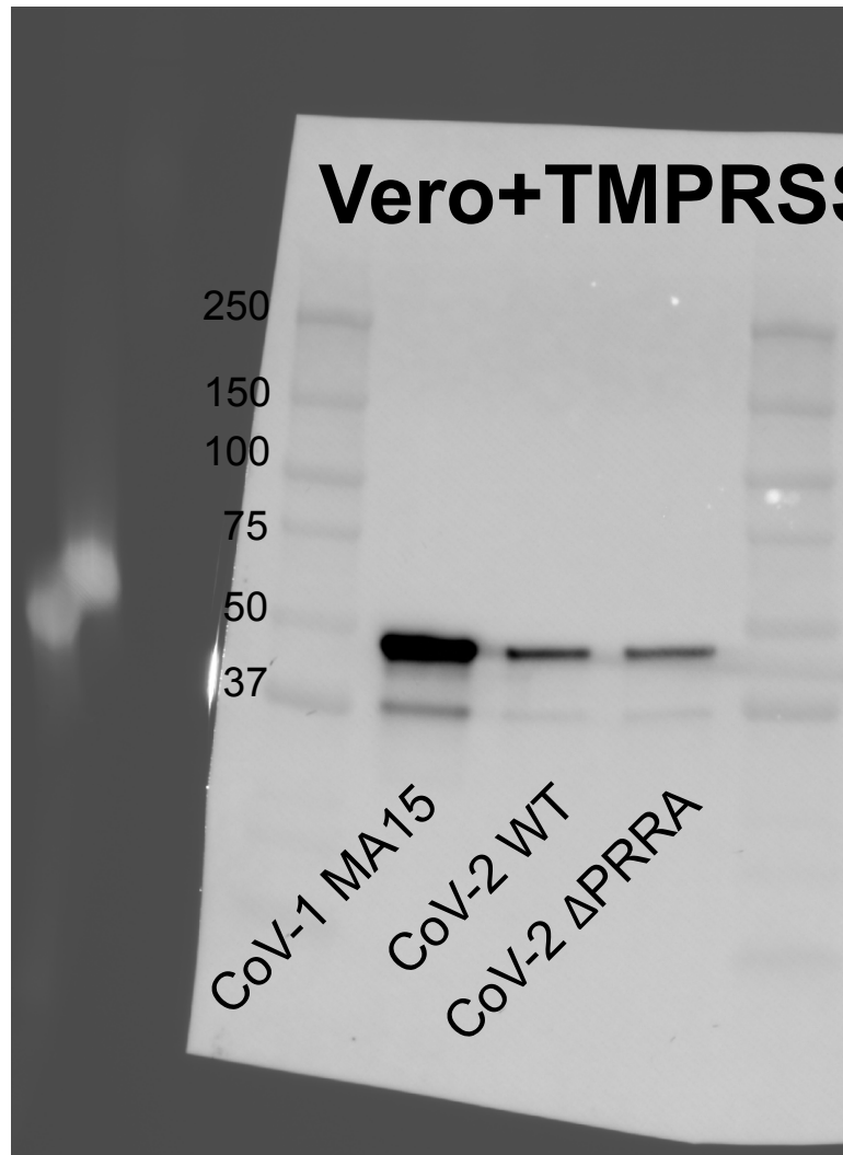
Supplementary Figure 4. Uncropped chemiluminescent images of Western blots for CoV Nucleocapsid proteins from bottom panels Figures 1j.
