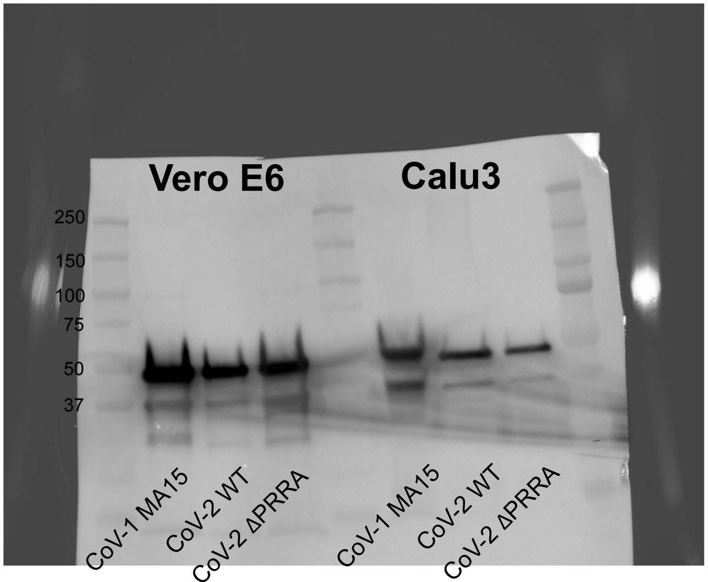
Supplementary Figure 2. Uncropped chemiluminescent images of Western blots for CoV Nucleocapsid proteins from bottom panels Figures 1d and 1g.
