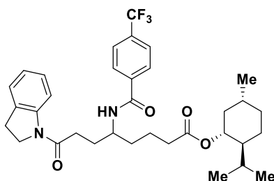
Figure 3, entry 40, (S,S)-N2*: 95:5 dr; (R,R)-N2*: 6:94 dr.
