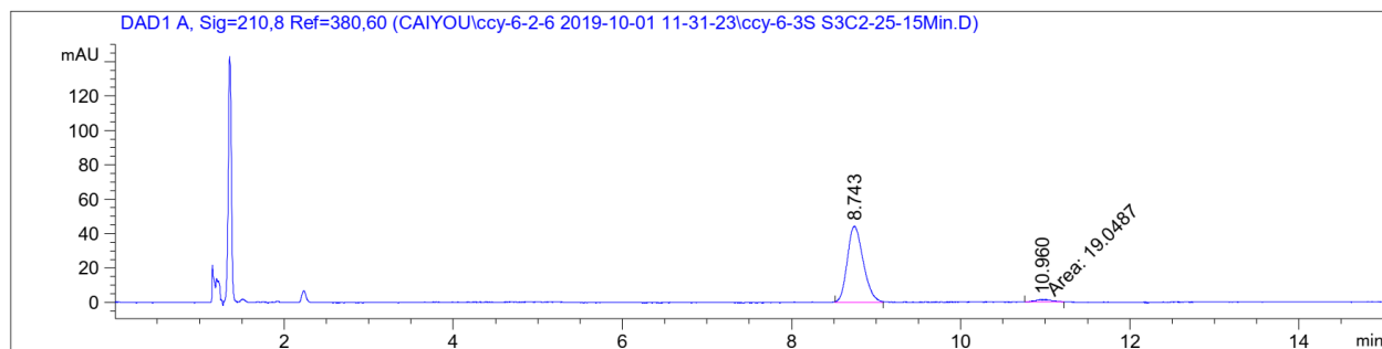
Figure 3, entry 37, (S,S)-N2*: 94% ee; (R,R)-N2*: 94% ee.
