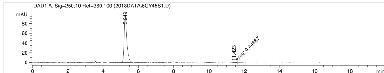
Figure 3, entry 63, ( S,S )-N1*: 98% ee; ( R,R )-N1*: 98% ee.
