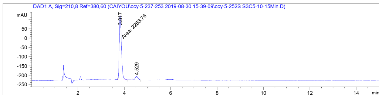
Figure 3, entry 27, ( S,S )-N1*: 88% ee; ( R,R )-N1*: 88% ee.
