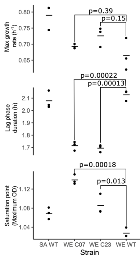
Supplementary Fig. 10 | Growth phenotypes of CDC36 promoter mutant strains. Maximum growth (y axis, top), duration of lag phase (y axis, middle) and saturation of growth (y axis, bottom) for two WT strains and two engineered strains (x axis). Bars: means, dots: replicate measurements. P-values: Student's t-test; two-sided, unpaired, equal variance. n=3 replicates/strain.
