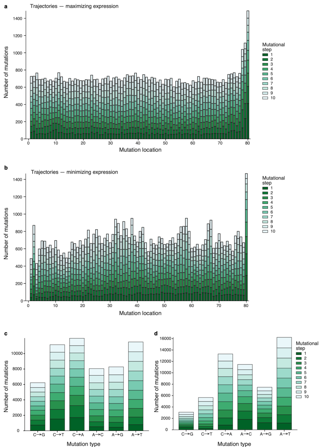
Supplementary Fig. 7 | Sequences took diverse paths to evolve extreme expression. a-b , The number (y axis) of mutations across each promoter position (x axis; -160 to -80 region) for trajectories under the SSWM regime starting with native promoter sequences when (a) maximizing or (b) minimizing expression in defined media using the convolutional model. Some of the observed bias to TSS-proximal mutations may be related to prior observations of proximal repressor activity bias(de Boer et al. , 2020). c,d , The number (y axis) of mutations of each type (x axis) for trajectories under the SSWM regime starting with native
