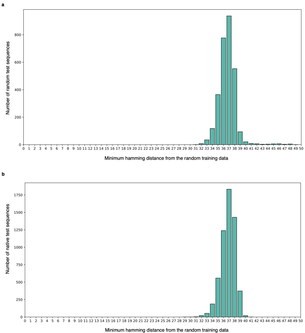
Supplementary Fig. 21 | Sequence differences between training and test data. The distribution of the Hamming distance between each sequence in the (a) random or (b) native test sets and the closest sequence in the random training set.
