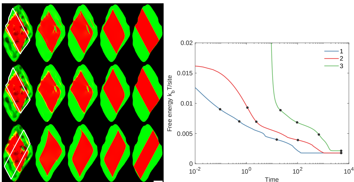
Figure S5: The experimental image of Li concentration field in relaxed LFP particles, and the simulated concentration field over time. The LFP-FP interface from the simulation at the last time step is shown on the experimental image as the white curve for comparison. The free energy evolution is plotted for all relaxation scenarios. Legend 1, 2, and 3 refer to the relaxation via diffusion, via reaction (starting from experimental image), and relaxation via reaction (starting from a uniform concentration field), and correspond to the 1st, 2nd, and 3rd rows. Black dots in the free energy curves correspond to the simulation snapshots shown. The scale bar is 500 nm. The image horizontal and vertical axes correspond to crystallographic a and c axes.
