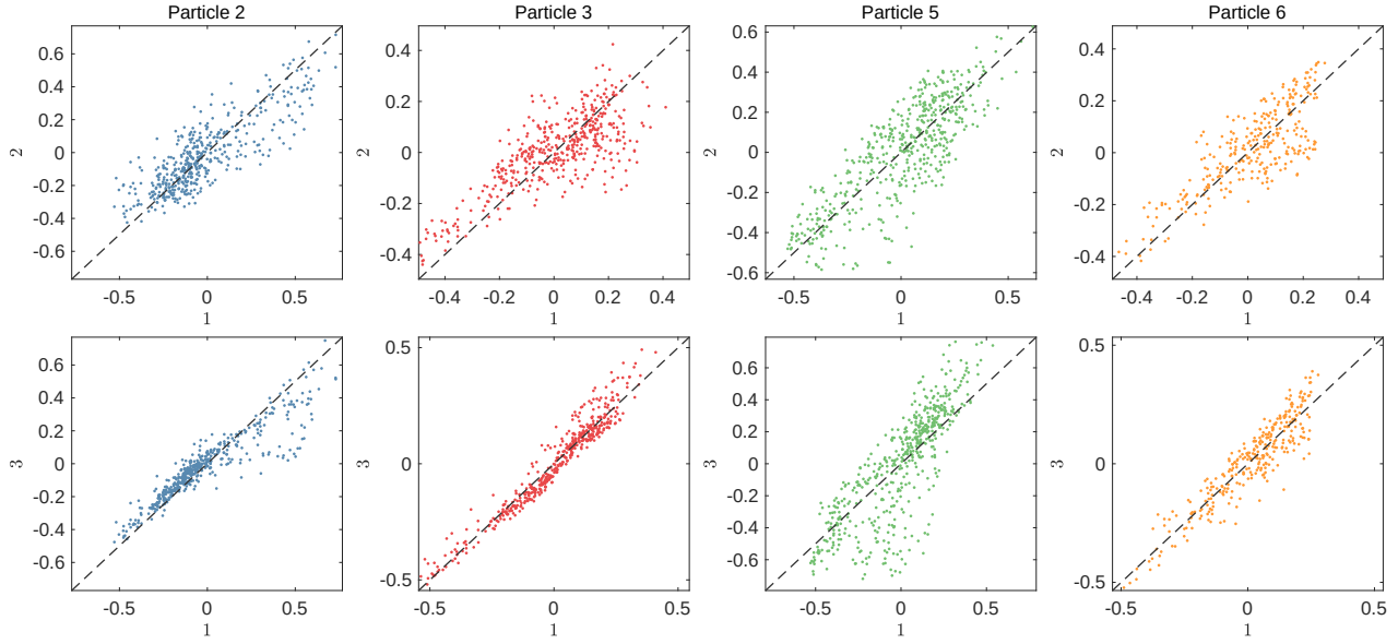
Figure S43: Pointwise correlation plots of centered \ln k(\mathbf{x}) from the k -fold validation for particles 2, 3, 5, and 6 when \rho_2 = 0.7 . The horizontal and vertical axis labels refer to which dataset is used for validation. The other two datasets are then used for training.
