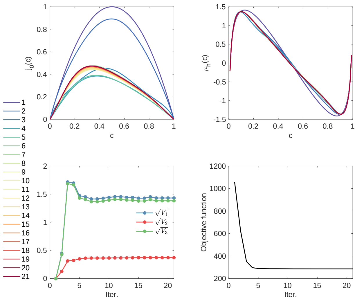
Figure S24: Optimization using trust-region algorithm.
