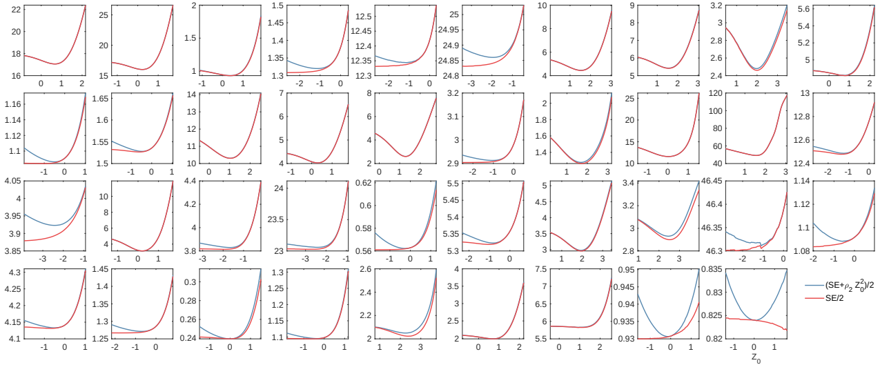
Figure S37: Squared error SE_i and (SE + \rho_2 Z_0^2)/2 of each particle (including all episodes) as a function of its respective Z_0 near the optimum when all other parameters are fixed.
