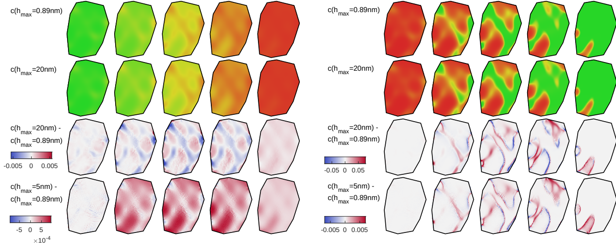
Figure S20: A comparison of solution using different mesh sizes at reaction rate R = 2 \text{ hr}^{-1} (left) and R = -0.3 \text{ hr}^{-1} (right). The first row is solved using a very fine mesh and is considered to be an approximation of the truth. The second row is the solution on a coarse mesh. The third and fourth rows are errors using different mesh sizes indicated on the left. All concentration and error fields are interpolated onto the same grid size ( 100 \times 136 ).
