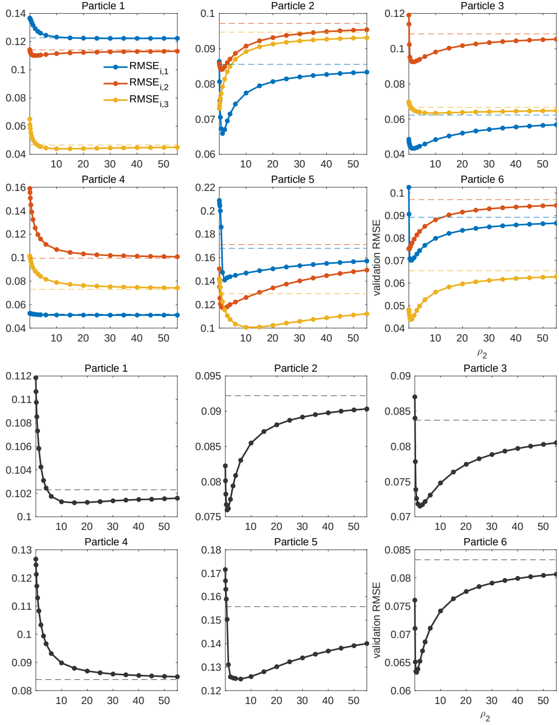
Figure S42: Top: the RMSE of each of the 3-fold validation of the particle RMSE i,j , where i = 1, \dots, 6 , corresponding to particle 1 to 6. Bottom: average validation RMSE of each particle RMSE i . The dashed lines are the asymptotic limit when \rho_2 = \infty , that is, when there is no spatial heterogeneity ( \ln k(\mathbf{x}) = 0 ).
