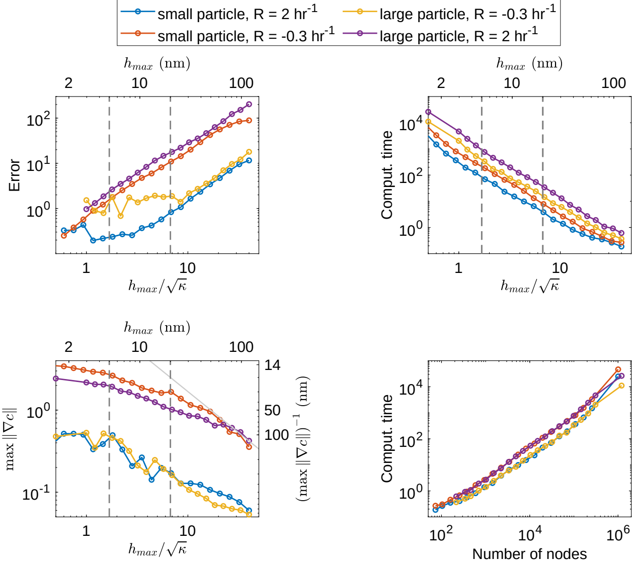
Figure S19: Error, computational time, and convergence analysis based on simulated data. The horizontal axis is the maximum mesh size h_{\max} normalized by \sqrt{\kappa} , or in physical unit nm, or the total number of nodes in the mesh. The dimensionless error and \|\nabla c\| are based on STXM pixel size. The areas for the small and large particles are 300 and 1000 pixels, respectively. The vertical dashed lines correspond to two sets of mesh used in performing forward simulation and inversion tests.
