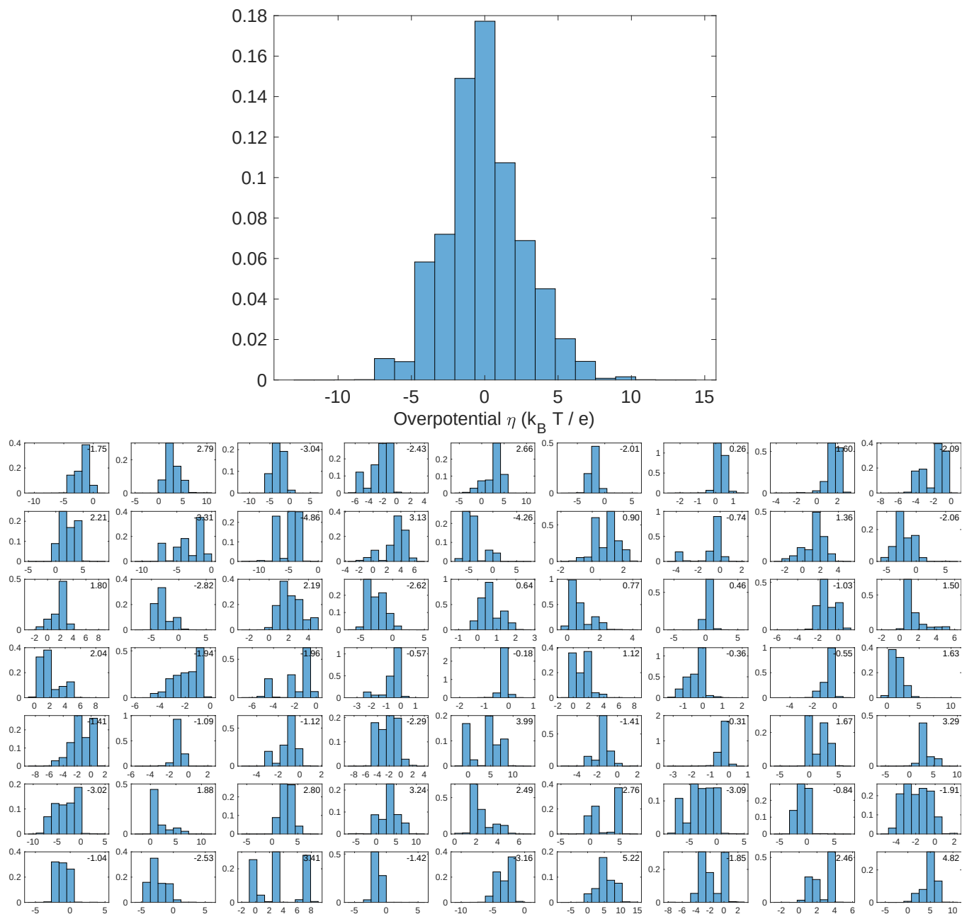
Figure S51: The histogram of overpotential (a) at all frames and pixel locations (b) for each episode when trained using all datasets and at the optimal regularization coefficient \rho_2 = 0.88 . The label is the mean overpotential of the episode.
