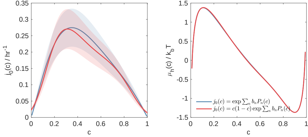
Figure S27: The MAP estimate of \mu_h(c) and j_0(c) and the 99% confidence interval estimated using the Hessian at MAP. Natural boundary condition is used for the model.
