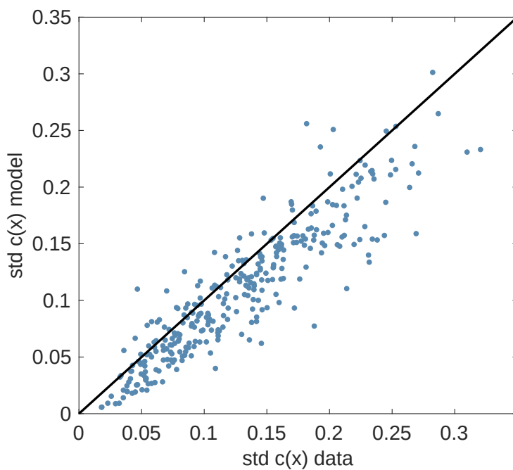
Figure S56: Standard deviation ( \text{std} = v^{1/2} ) of c(x) of all frames between data and learned model.
