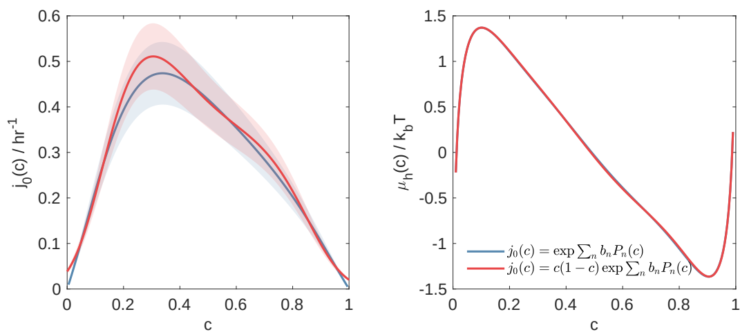
Figure S30: The MAP estimate of \mu_h(c) and j_0(c) and the 99% confidence interval estimated using the Hessian at MAP. The essential boundary condition is used for the model.
