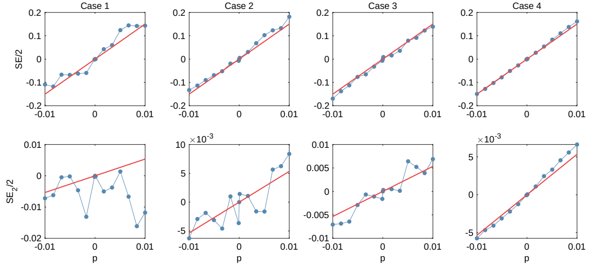
Figure S17: The objective function landscape in the direction of the second parameter for \mu_h(c) . The objective function and parameter are centered so that they are zero at the nominal parameters. The blue lines with markers correspond to the function value at discrete points. The red lines correspond to the tangent line at p = 0 computed by the adjoint sensitivity analysis. See the main text for the description of the different cases.
