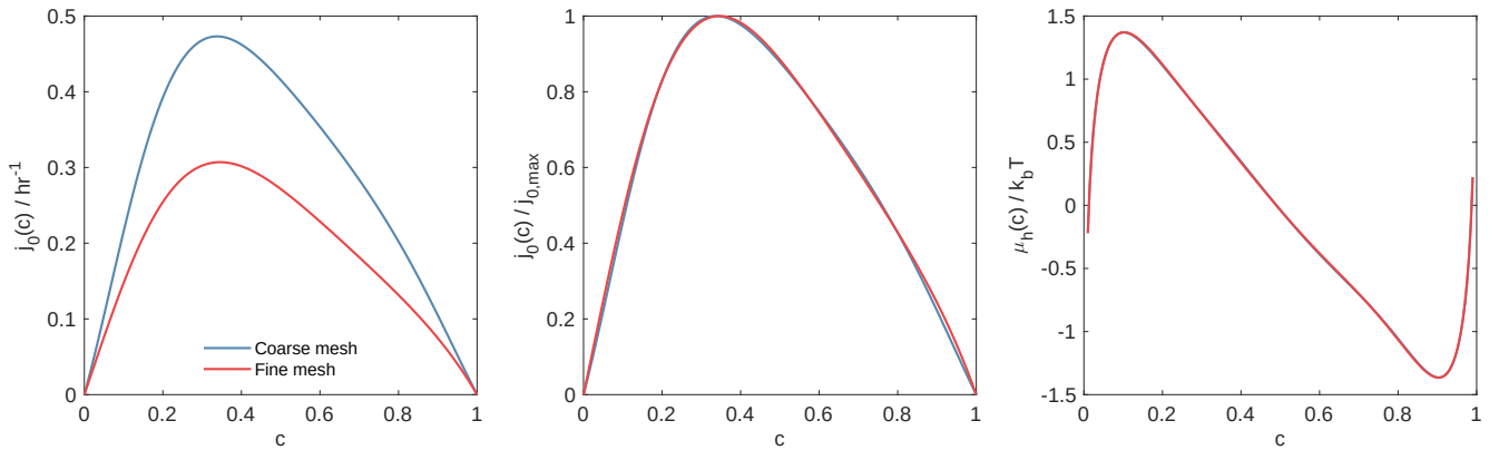
Figure S21: The MAP estimate of \mu_h(c) and j_0(c) using a coarse (maximum mesh size equals 40% pixel size, or 20 nm) and fine mesh (maximum mesh size equals 10% pixel size, or 5 nm).
