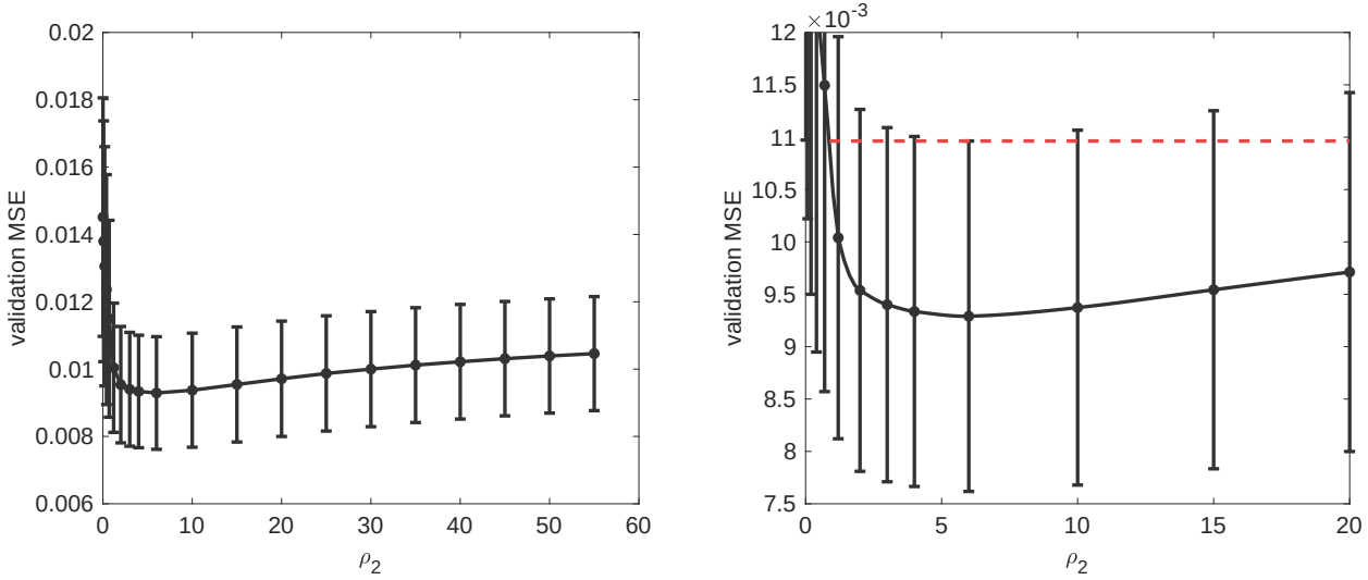
Figure S41: The sample mean and standard deviation of the validation mean squared error \text{MSE}_{\mathcal{V}} as a function of the regularization coefficient \rho_2 . The right plot is a zoom-in view of the left plot.
