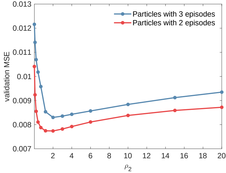
Figure S44: The validation WSE for particles with 3 episodes and 2 episodes as a function of \rho_2 .
