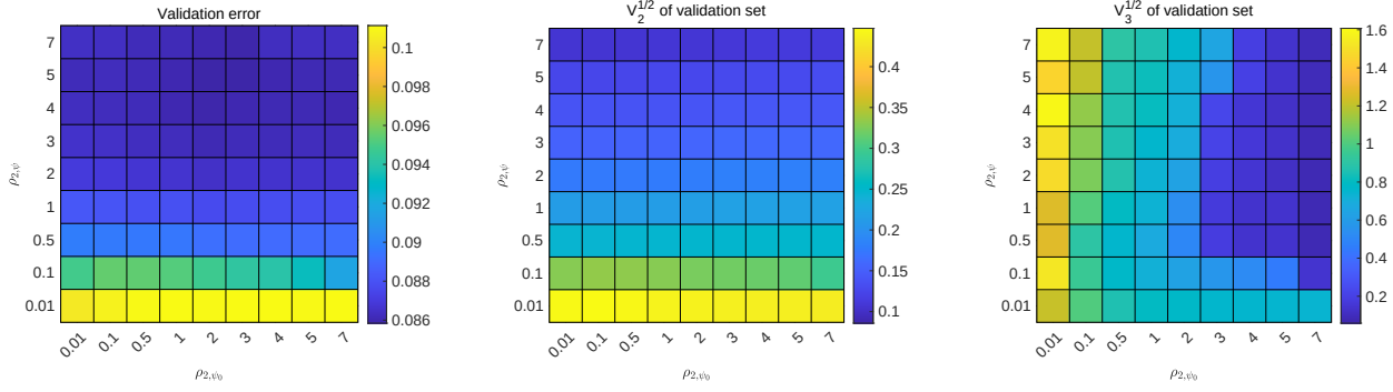
Figure S38: The validation error, intraparticle variation V_2^{1/2} , and interparticle variation V_3^{1/2} of the validation dataset when \rho_{2,\psi_0} and \rho_{2,\psi} , the regularization coefficients on Z_0 and Z_{i \neq 0} respectively, varies independently.
