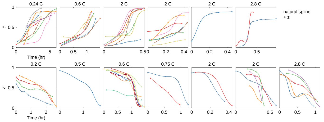
Figure S26: The average Li composition from experimental data (dots) and the interpolated trajectory using spline on the transformed variable z .
