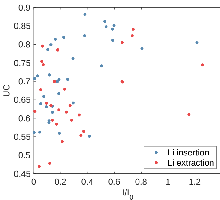
Figure S55: The uniformity coefficient of each episode computed from image data versus I/I_0 .
