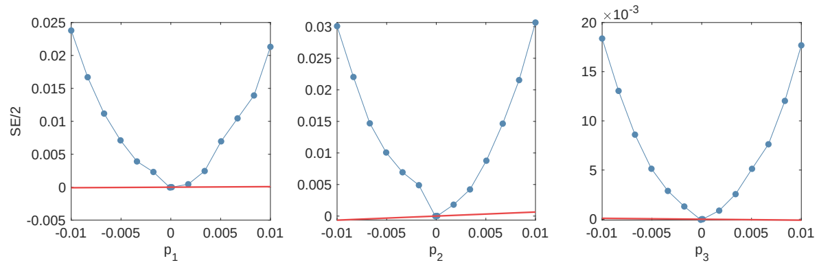
Figure S18: The objective function as a function of the three parameters of \mu_h(c) at the optimum found by the optimizer. The blue lines with markers correspond to the function value at discrete points. The red lines correspond to the tangent line at p = 0 computed by the adjoint sensitivity analysis. Both are evaluated using \text{RelTol} = 5 \times 10^{-4} and \text{AbsTol} = 10^{-4} and reinitialization at each frame.
