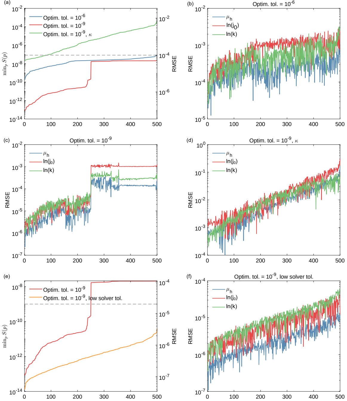
Figure S32: The optimization results starting from 500 randomly chosen initial guesses. (a) The sorted final objective function S(\mathbf{p}) and RMSE of c(\mathbf{x}) when the DAE solver relative and absolute tolerance is 10^{-3} and 10^{-4} . A comparison of high and low optimizer tolerance and when \kappa is or is not included as a free parameter. The dashed line corresponds to the absolute tolerance of the DAE solver. (b,c,d) the RMSE of \mu_h(c) , j_0(c) , and k(\mathbf{x}) that correspond to the sorted objective function in (a). (e) The sorted final objective function S(\mathbf{p}) and RMSE of c(\mathbf{x}) when the optimizer tolerance is 10^{-9} , a comparison of high and low solver tolerance. The dashed line corresponds to the optimizer tolerance. (f) the RMSE of \mu_h(c) , j_0(c) , and k(\mathbf{x}) that correspond to the sorted objective function in (e).
