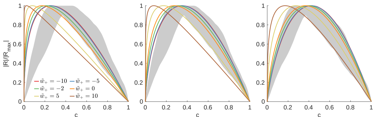
Figure S53: Comparison of |R(c, \eta)|/| \max_c R(c, \eta) | predicted by CIET at \eta = 2.5k_B T/e , a_+ = 0.015 and various values of surface adsorption energy \tilde{w}_+ = w_+/k_B T with the inferred reaction kinetics based on Butler-Volmer kinetics.
