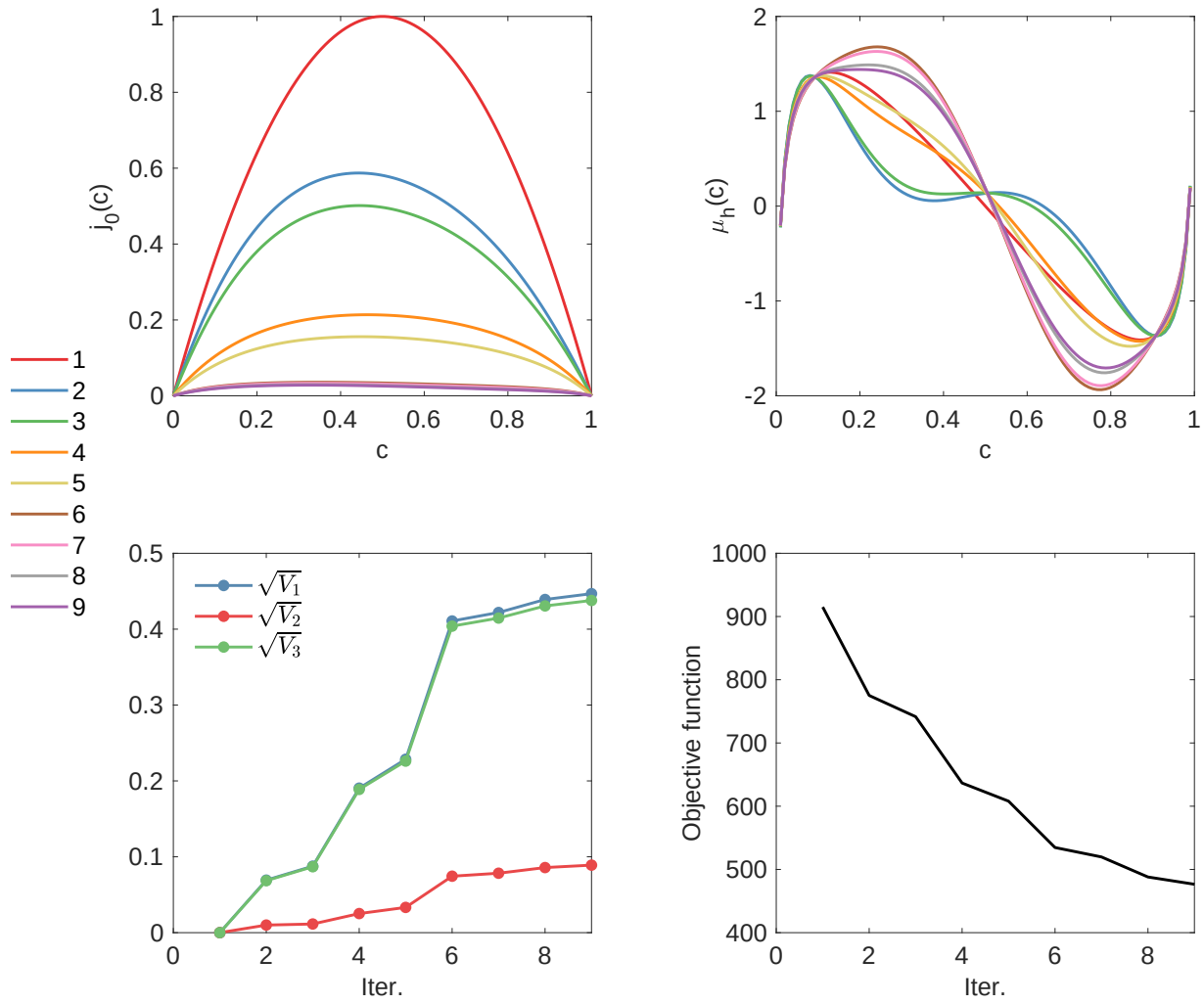
Figure S23: Optimization using quasi-Newton algorithm. j_0(c) , \mu_h(c) , variance of \ln k(\mathbf{x}) , and the objective function at each iteration during optimization is shown. See the legend on the left for the color of each iteration.
