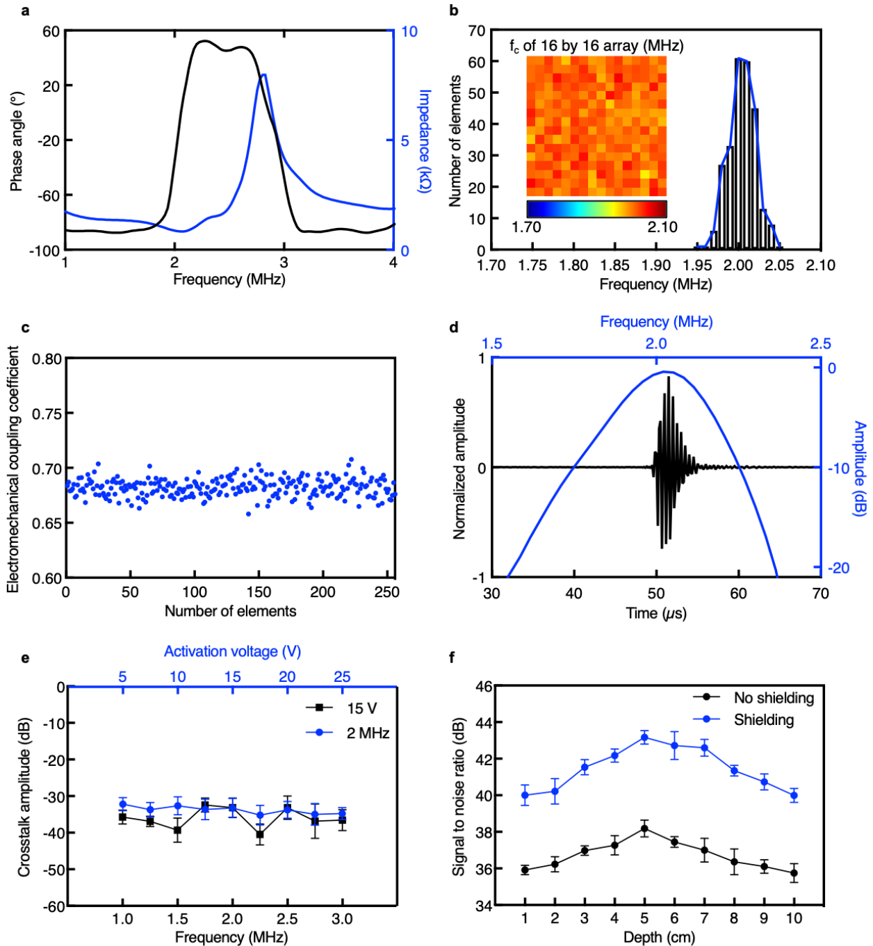
Supplementary Fig. 8 | Characterizations of the conformal ultrasound patch. a , Phase angle and electrical impedance spectra from 1 MHz to 4 MHz. The center frequency is 2.01 MHz with a phase angle of 11.96°. b , The center frequency distribution among the 256 elements of the patch. Inset is its distribution map of the 16 by 16 array. c , The electromechanical coupling coefficient of the 256 elements. d , Pulse-echo response and corresponding frequency spectra of a typical element. The measured -6 dB bandwidth is 17.41%. Doppler signal processing requires extracting Doppler shift in the frequency domain. The small bandwidth provides sharper peaks in the frequency domain. Thus, the frequency difference between transmitted and received signals can be calculated more easily. e , Crosstalk between adjacent transducer elements for both frequency sweep and
