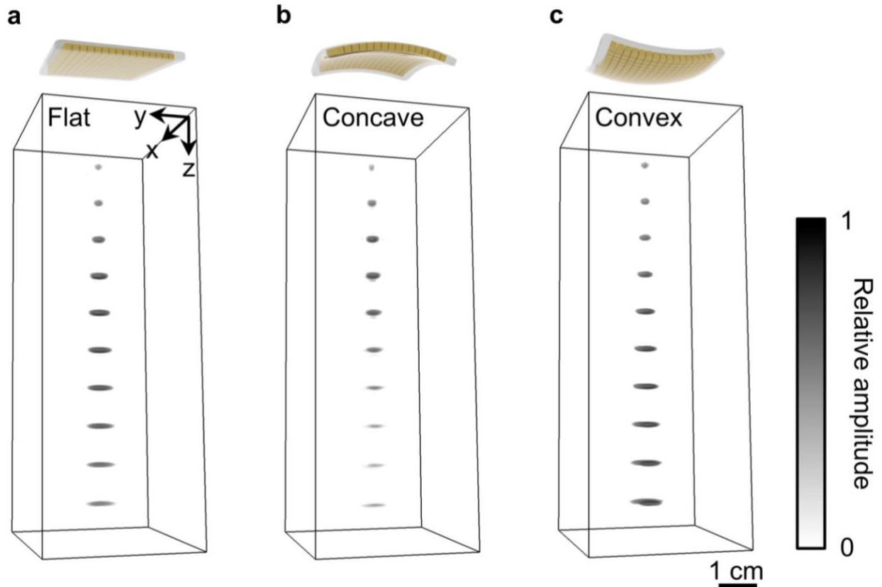
Supplementary Fig. 9 | Simulated 3D images of point phantoms for the patch under different configurations. When the conformal ultrasound patch is attached to the skin, it may cause deformation of the transducer array, which could subsequently result in phase aberration, particularly at high frequencies. However, the ultrasound patch operates at a relatively low frequency of 2 MHz in this study, which has a much higher tolerance for phase aberration. We performed a simulation to illustrate that the skin curvature has a very low influence on the beamforming for low-frequency arrays using the Matlab Field II toolbox. We placed a 2 MHz soft array on a , flat, b , concave, and c , convex surfaces. The radii of curvature for the concave and convex are both 5 cm. A coherent compounding imaging strategy with 5 insonification angles and an interval of 5^\circ is used. The simulation phantom comprises 10 points extending from a depth of 1 cm, with each subsequent point deeper by 1 cm. Simulation results show that for the concave array, the shallow points have higher amplitudes, while the deep points have lower amplitudes, than the flat array. This is because the concave array emits a more focused sound beam compared to the flat array, resulting in higher sound field intensity at a shallower depth. For the convex array, the sound beam is more diverged than the flat array. Therefore, the signal amplitudes are a bit lower than the flat array, and the reconstructed points are a bit larger. Albeit these differences in intensity and resolution, they are still within an acceptable range. The images share the same scale bars.
