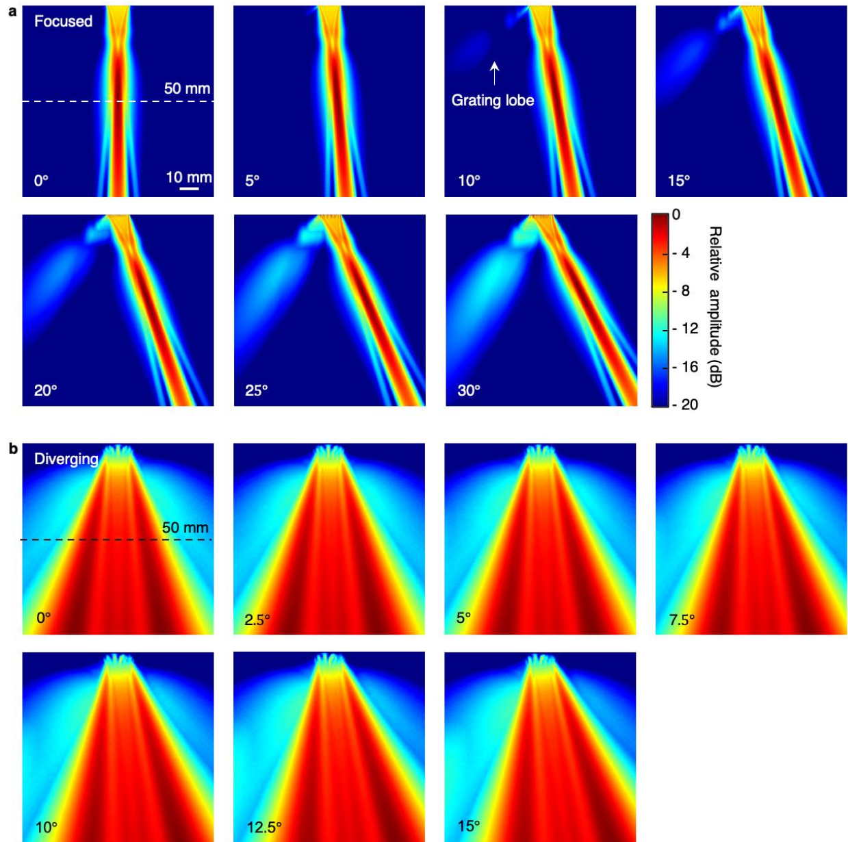
Supplementary Fig. 6 | Simulated ultrasound beam steering. a , Ultrasound waves focus at 50 mm depth with a beam tilting angle of 0°, 5°, 10°, 15°, 20°, 25°, and 30°, respectively. The grating lobe is growing and becomes more obvious when the beam tilting angle is larger. b , Diverging ultrasound waves with a beam tilting angle of 0°, 2.5°, 5°, 7.5°, 10°, 12.5°, and 15°, respectively. The simulation was performed using an open-source Matlab toolbox Field II. The medium was set as uniform with a sound speed of 1,540 m/s and a density of 1,000 kg/m 3 . The central frequency was 2 MHz, the same as the real probe. We applied the built-in function, “ xdc_2d_array ”, to create the transducer array. The transmitted waveform from each transducer element could be set to be a focused beam or a diverged beam. All simulation results share the same scale bars.
