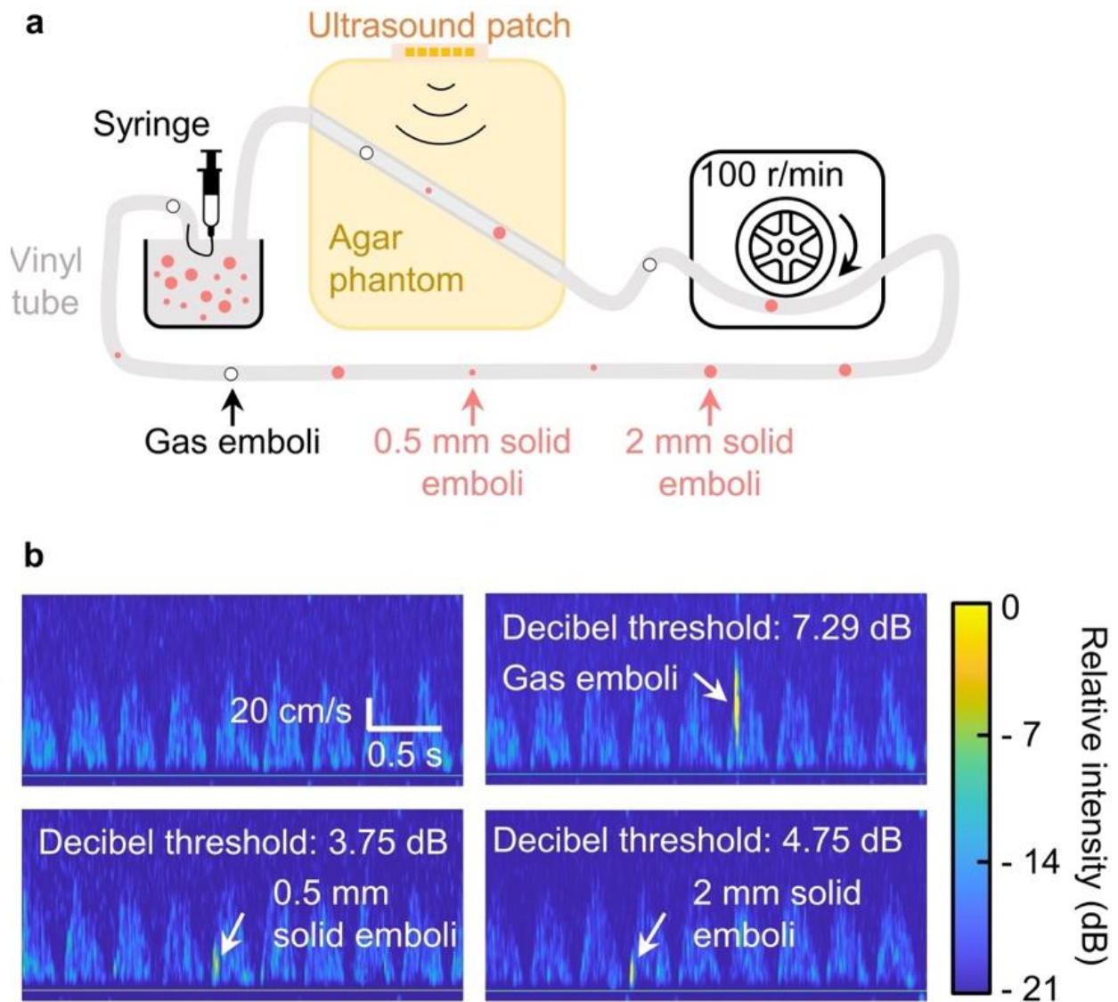
Supplementary Fig. 57 | Conformal ultrasound patch for emboli detection on phantom. a, Schematic experimental setup. Three different types of emboli are used, including gas emboli, 0.5 mm solid emboli, and 2 mm solid emboli. b, Flow spectra of baseline, with gas emboli, with 0.5 mm solid emboli, and with 2 mm solid emboli, respectively. The spectra share the same scale bars.
