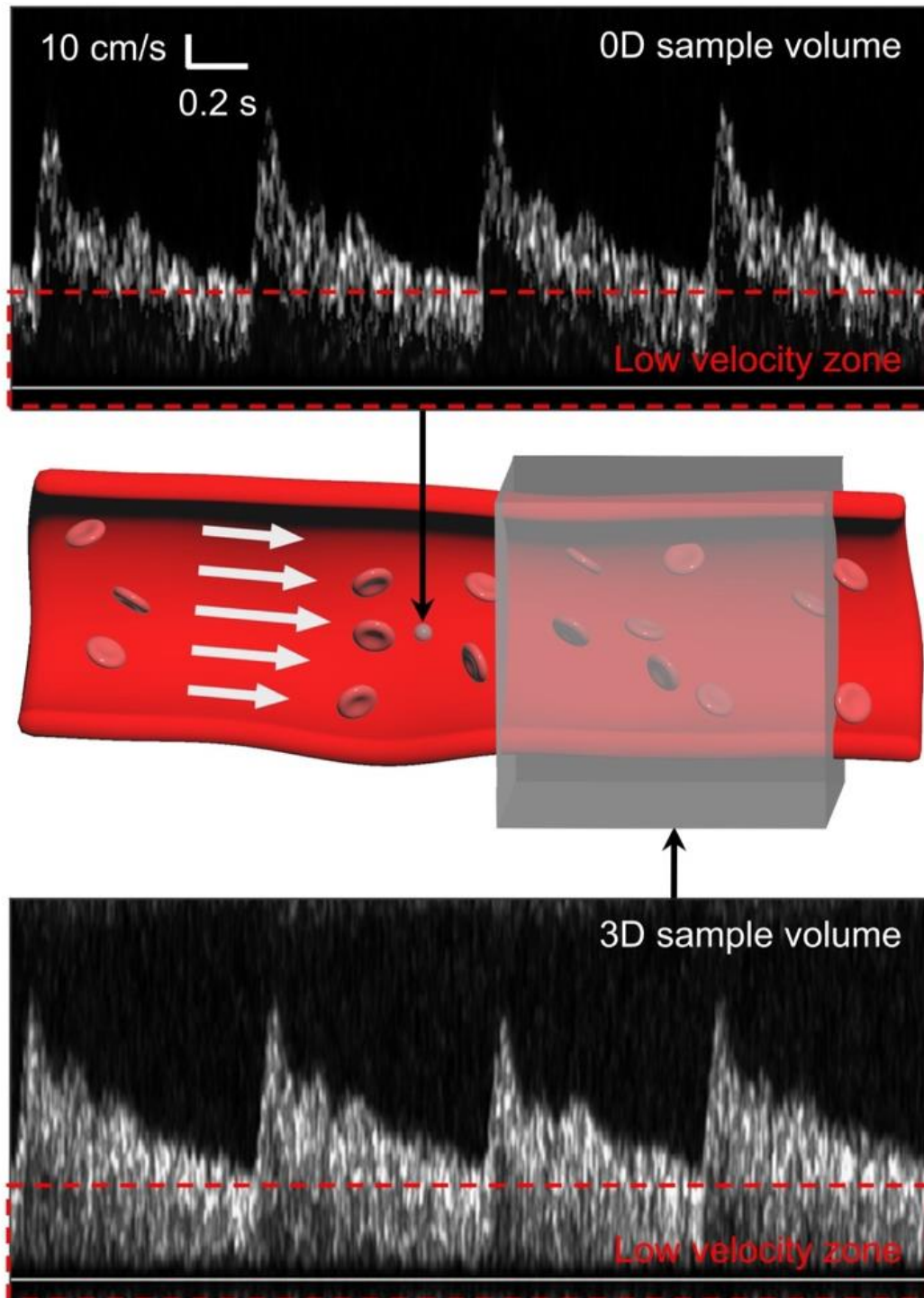
Supplementary Fig. 51 | Sample volume optimization. The comparison of blood flow spectra from different sample volumes. The 0D sample volume (single pixel, around 0.77 \times 0.77 \times 0.77 \text{ mm}^3 ) only contains partial blood flow distributions, while the 3D sample volume (216 pixels, around 4.62 \times 4.62 \times 4.62 \text{ mm}^3 ) contains the entire blood flow distributions of the target blood vessel segment. For patients with cerebral arterial diseases such as stenosis, the turbulence flow pattern may happen in the zone of low frequency shift (i.e., low blood flow velocity), which can be seen only if an appropriate 3D sample volume is selected. The spectra share the same scale bars.
