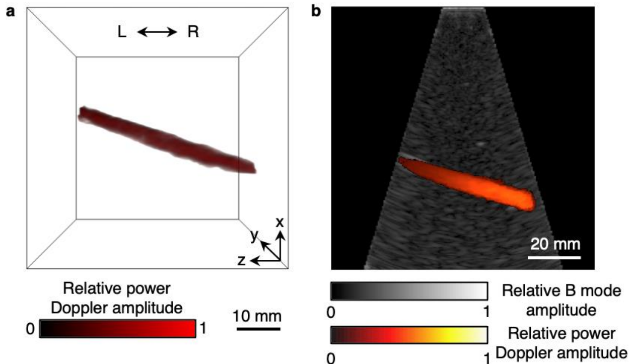
Supplementary Fig. 59 | Characterization of flow in an arterial phantom. We pumped Doppler fluid (769DF, CIRS) through a Doppler flow phantom (ATS 523A, CIRS) with 4 mm in diameter at an approximate depth of 60-80 mm. The figure shows volumetric flow imaging results from the ultrasound patch alongside the ground truth obtained by a commercial ultrasound probe (e.g., a P4_2v phased array probe) using duplex mode (B mode and power Doppler mode) imaging. a , A volumetric image of the flow in the phantom captured by the ultrasound patch. b , The ground truth collected by the commercial ultrasound probe. These results demonstrate that the vessel structure measurement from the ultrasound patch is consistent with that from conventional imaging devices, validating its accuracy in capturing blood flow dynamics. L, left. R, right.
