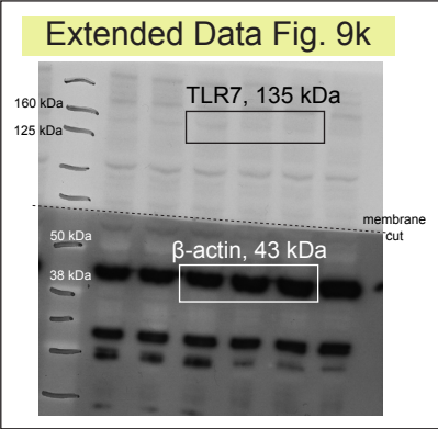
Supplementary Figure 1. Uncropped Western blot scans.
