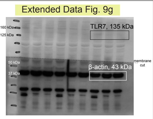
Supplementary Figure 1. Uncropped Western blot scans.
