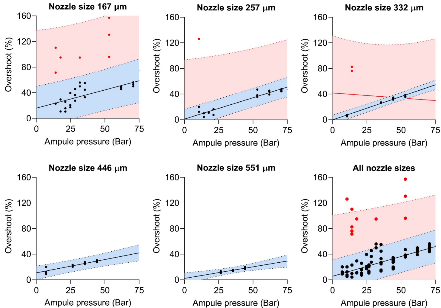
Supplementary fig. 2: Linear regressions of overshoot results.
