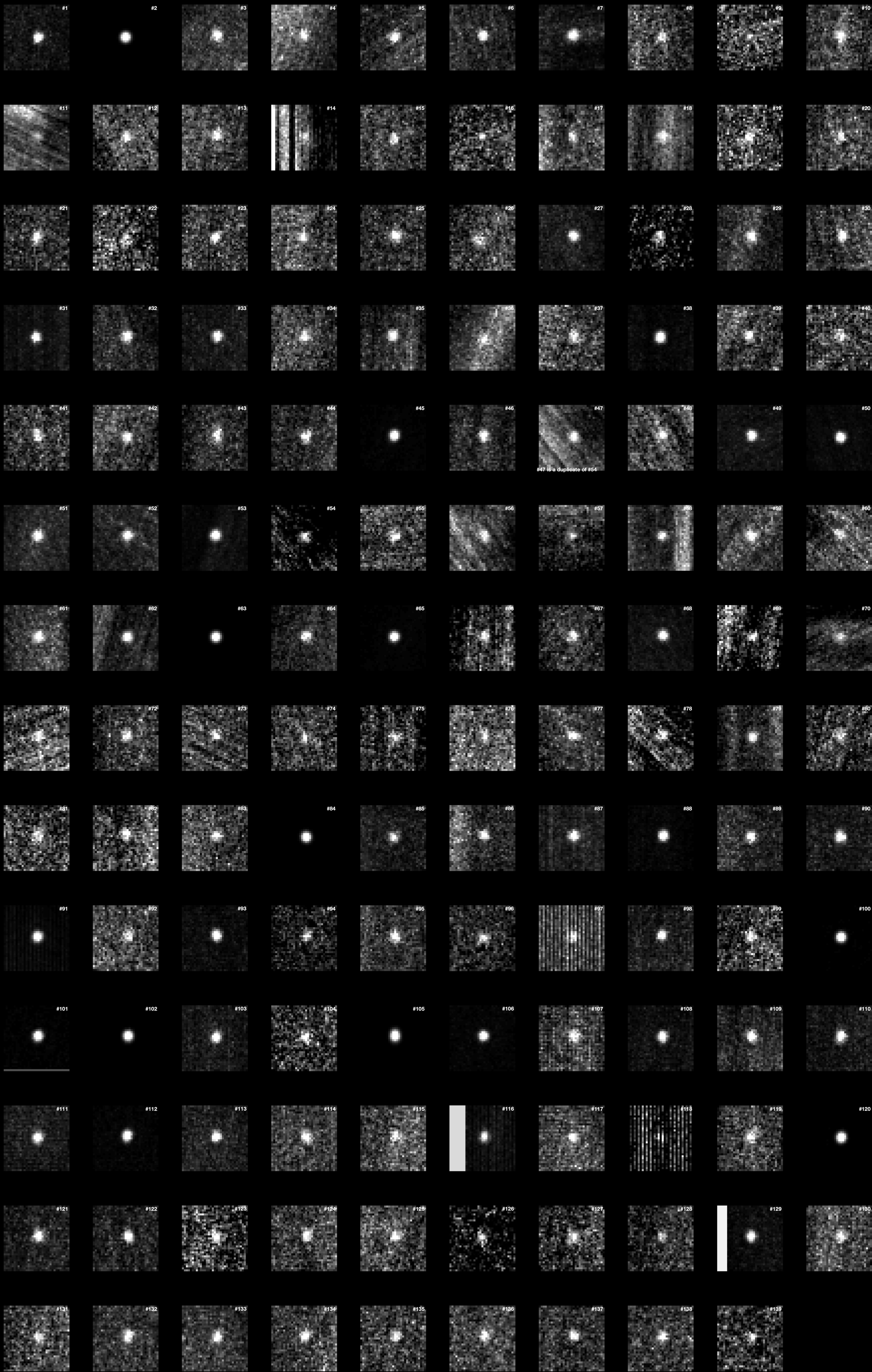
Family portait of the 138 new JWST asteroids fom Burdanov, de Wit, et al. 2024
