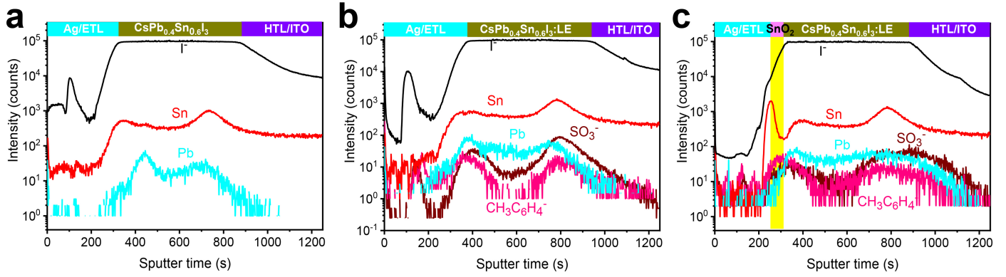
Extended Data Fig. 4 | ToF-SIMS measurements. ToF-SIMS of depth profiles of anion distribution in inorganic (a) CsPb 0.4 Sn 0.6 I 3 , (b) CsPb 0.4 Sn 0.6 I 3 :LE and (c) CsPb 0.4 Sn 0.6 I 3 :LE based on ALD-SnO 2 PSCs with continuous illumination at 85 °C for 10 days in N 2 glovebox.
