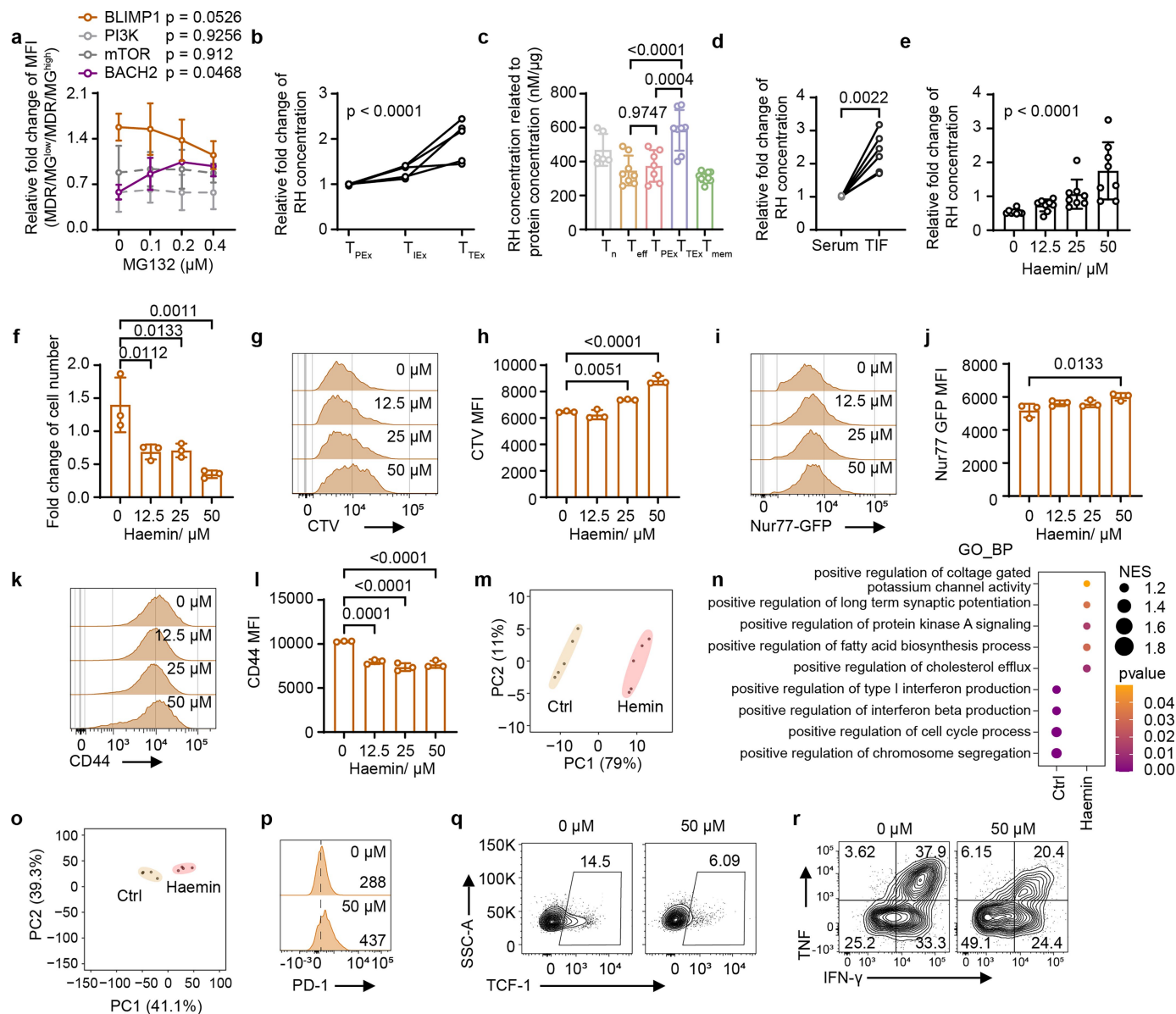
Extended Data Fig. 3 | Haem released due to the mitochondrial protein degradation instructs terminal differentiation.
