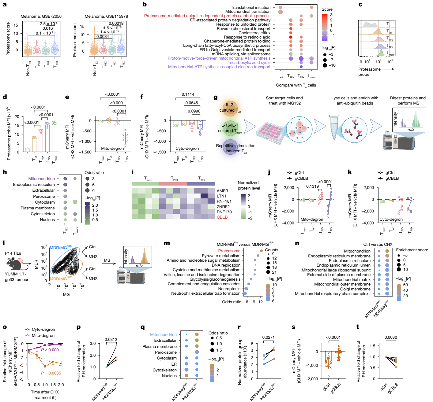
Fig.1 | Proteasome-mediated mitochondrial protein degradation.
