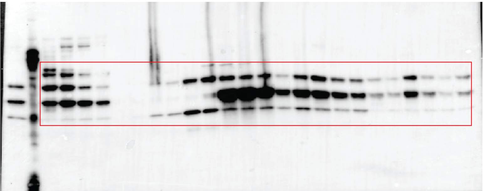
143B m.1227G>A Sucrose Gradient MRPS14
