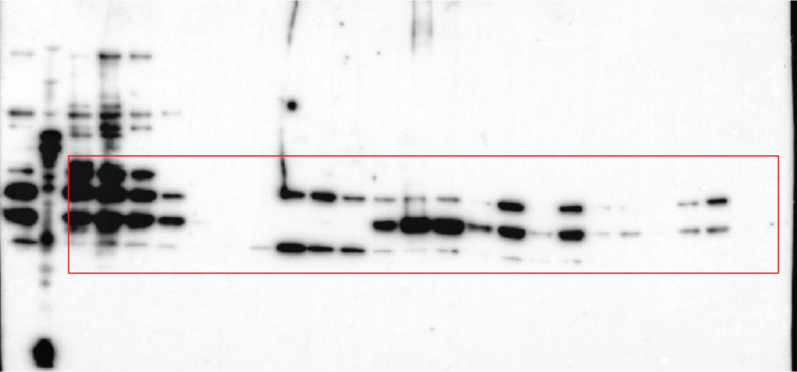
143B WT Sucrose Gradient MRPS27, MRPL44, MRPS34
