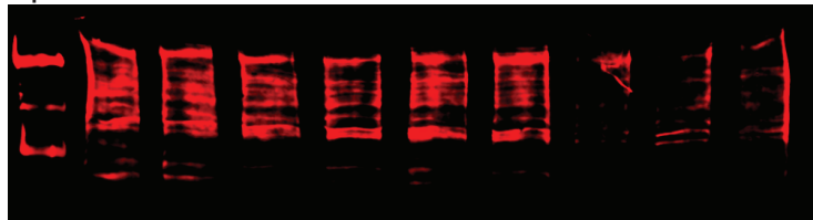
Input: Multiplexed (single acquisition) DNMT1 + SUMO2/3
