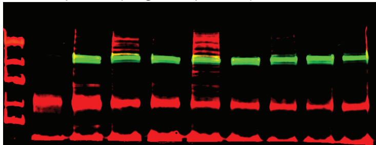
IP: Multiplexed (single-acquisition) DNMT1 + SUMO2/3
