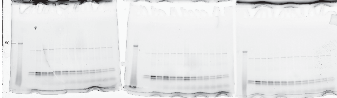
BarstarK78 unmodified ubiquitin-independent degradations. Triplicate trials. Fluorescein imaged.
