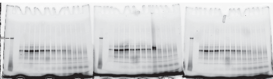
BarstarK60 Mono-ub ubiquitin-independent degradations. Triplicate trials. Fluorescein imaged.
