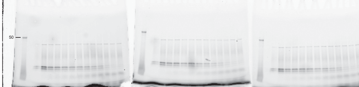
BarstarK60 unmodified ubiquitin-independent degradations. Triplicate trials. Fluorescein imaged.
