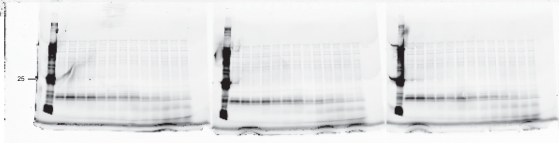
BarstarK2 unmodified ubiquitin-independent degradations. Triplicate trials. Fluorescein imaged.
