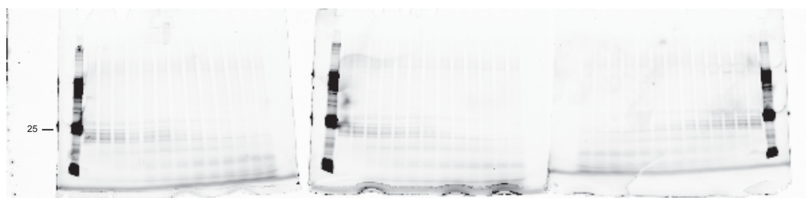
BarstarK2 Mono-ub ubiquitin-independent degradations. Triplicate trials. Fluorescein imaged.
