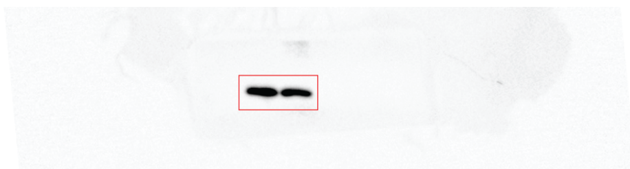
Uncropped image of Chemiluminescence scan in reference to Extended Data Fig. 6d (IB: TRMT112).
