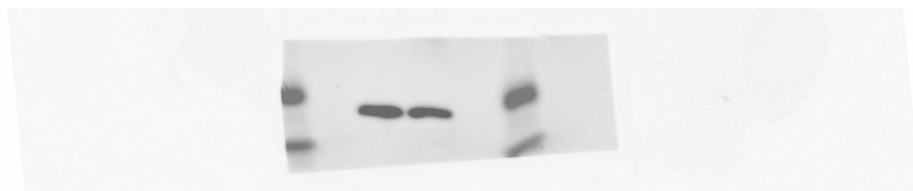
Uncropped composite image of Cy5 and Chemiluminescence scan in reference to Extended Data Fig. 6d (IB: TRMT112).
