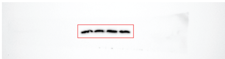
Uncropped image of Chemiluminescence scan in reference to Extended Data Fig. 6f (IB: TRMT112).
