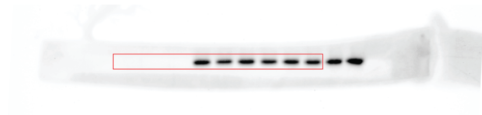
Uncropped image of Chemiluminescence scan in reference to Extended Data Fig. 6c (IB: HA).
