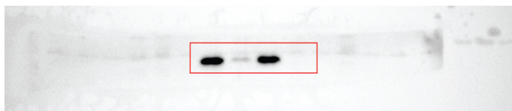
Uncropped image of Chemiluminescence scan in reference to Extended Data Fig. 6f (IB: METTL5).
