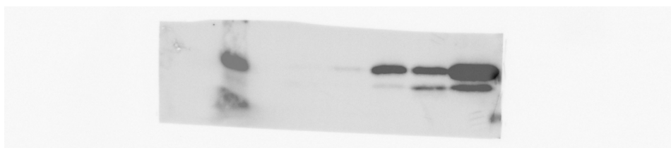
Uncropped composite image of Cy5 and Chemiluminescence scan in reference to Extended Data Fig. 6b (IB: TRMT112).
