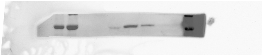
Uncropped composite image of Cy5 and Chemiluminescence scan in reference to Extended Data Fig. 6b (IB: ALKBH8).
