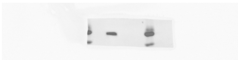
Uncropped composite image of Cy5 and Chemiluminescence scan in reference to Extended Data Fig. 6d (IB: METTL5).
