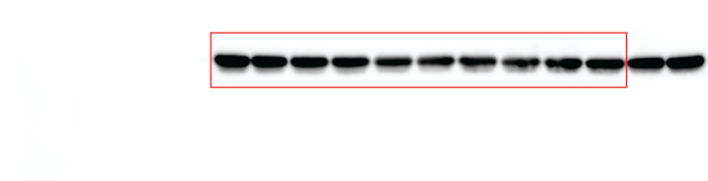
Uncropped image of Chemiluminescence scan in reference to Extended Data Fig. 6c (IB: \beta -actin).
