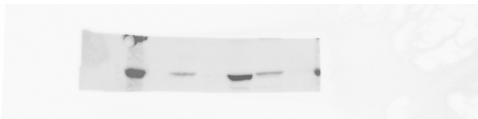
Uncropped composite image of Cy5 and Chemiluminescence scan in reference to Extended Data Fig. 6b (IB: TRMT11).
