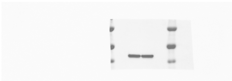
Uncropped composite image of Cy5 and Chemiluminescence scan in reference to Extended Data Fig. 6d (IB: \beta -actin).
