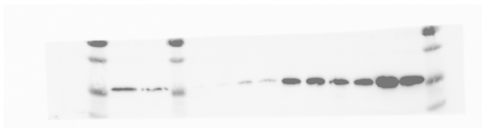
Uncropped composite image of Cy5 and Chemiluminescence scan in reference to Extended Data Fig. 6a (IB: FLAG, long exposure).
