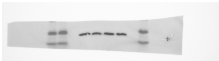
Uncropped composite image of Cy5 and Chemiluminescence scan in reference to Extended Data Fig. 6f (IB: TRMT112).
