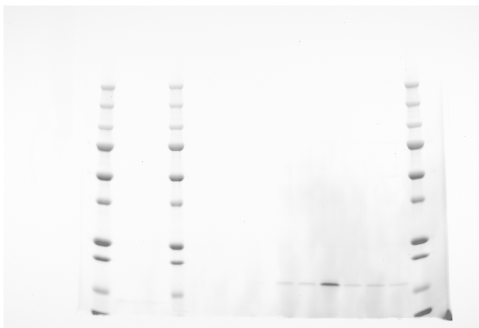
Uncropped composite image of Cy5 and Rhodamine scan in reference to Extended Data Fig. 6a (ABPP).
