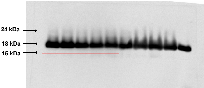
Total H3
