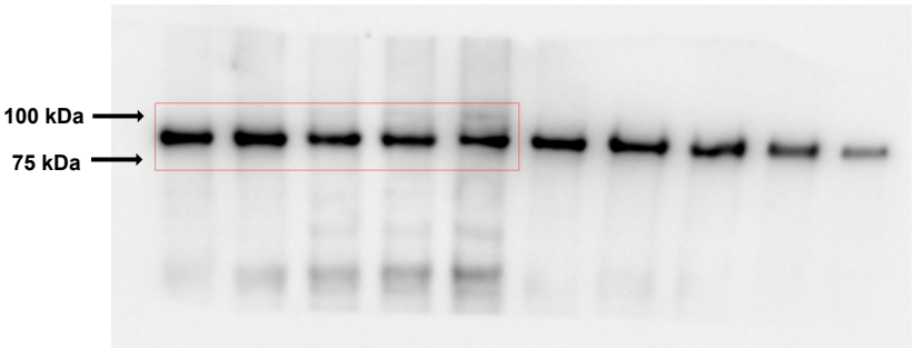
\beta -catenin
