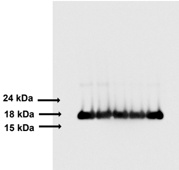
Total H3
