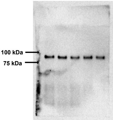
\beta -catenin
