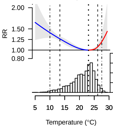
Toledo, Brasil Mean temp. 21C
