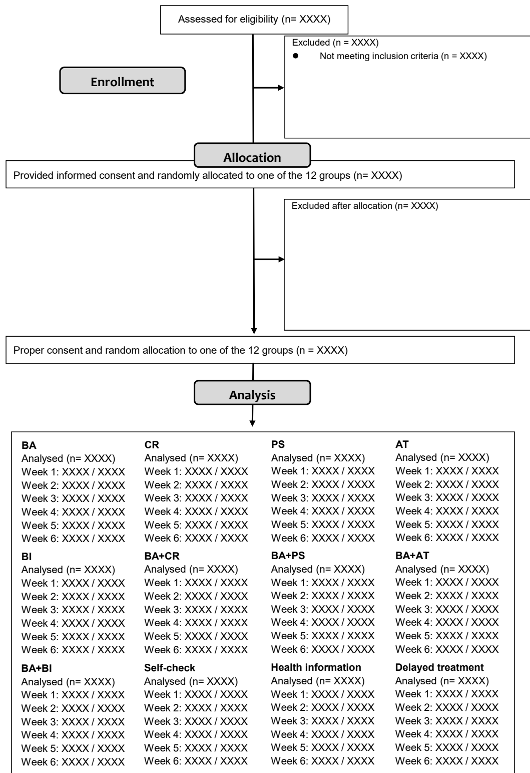
Figure 1. CONSORT diagram
