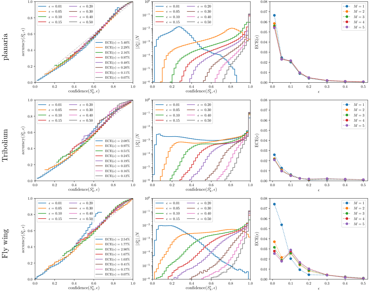
Supplementary Figure 26: Uncertainty evaluation of CARE network ensembles. Given an interval around each predicted restored pixel value (with size based on \epsilon ), we count a success if the true value is indeed contained in the interval. Furthermore, we compute the confidence of the ensemble as the probability that the true value will fall into this interval. The predicted per-pixel distributions are well-calibrated if the accuracy, i.e. the fraction of successfully predicted pixels, is close to the average confidence. Furthermore, we compare confidence and accuracy more granularly for subsets of pixels within a certain confidence range. For each of these subsets, we plot average confidence vs. accuracy, which gives rise to a reliability diagram (left column); note that we do this for intervals of various sizes as defined by \epsilon . The network ensemble is well-calibrated if the plotted curves are close to the identity function (dashed, gray). Additionally, we measure the expected calibration error (ECE) , which is essentially the average (weighted) difference of a curve to the identity function. The middle column shows the fraction of pixels that fall into each of the confidence ranges. The right column shows the expected calibration error as a function of interval size \epsilon for ensembles of sizes M = 1, \dots, 5 .
