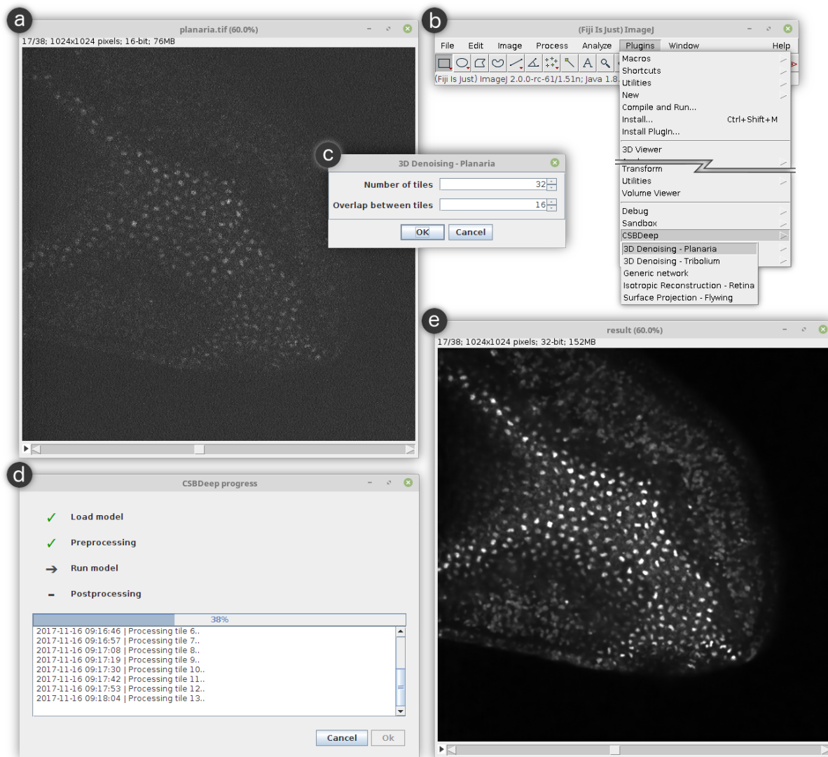
Supplementary Figure 29: FIJI integration of an example denoising workflow. (a) is a raw input image, loaded in FIJI. (b) the adequate plugin can be started from FIJI's menu Plugins \triangleright CSBDeep . (c) FIJI asks the user in how many tiles the input image should be subdivided for processing (see Section 5 for details). (d) the started CSBDeep plugin shows progress and status messages during execution of the network. (e) once terminated, the final result is shown in a separate FIJI window.
