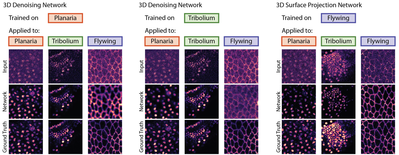
Supplementary Figure 24: Cross-application of trained CARE networks. For the planaria, Tribolium, and fly wing data we applied the respective trained network on images of all three data sets. As can be seen, the restoration quality drops in cases of mismatching training and test data ( e.g. planaria model on fly wing data). Interestingly, the amount of ‘hallucinated’ structures is negligible. Note that for the two denoising networks we show a slice through the resulting 3D volume, whereas the surface projection network results in a 2D projection of the whole input volume.
