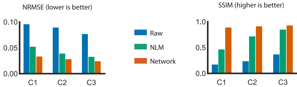
Supplementary Figure 7: Restoration of low-SNR images of Tribolium castaneum (flour beetle). Spinning disk confocal acquisitions of a developing embryo (EFA::nGFP labeling) at 3 different low-SNR conditions (C1-C3) and a high-SNR condition (GT). (a) Depicted are insets of the input, the best Non-Local-means (NLM) denoising result, the network reconstruction and the high-SNR ground-truth at different positions and tissue depth. (b) Reconstruction accuracy measured on held out test set (comprising 6 volumetric stacks for each condition). Shown are normalized root mean squared error (NRMSE, lower is better) and structural similarity (SSIM, higher is better). Note, that the parameters of the NLM baseline were optimized on the test-set, which would normally not be possible.
