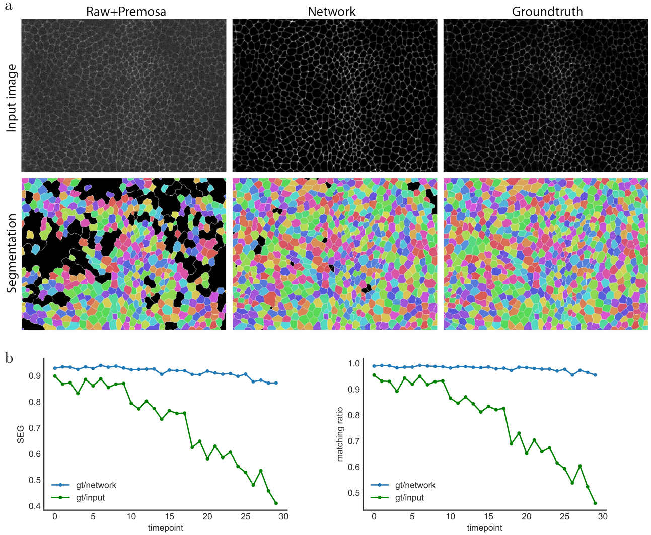
Supplementary Figure 12: Cell segmentation and tracking of a projected time-lapse of developing Drosophila melanogaster wing epithelia. (a) From left to right (upper row): Surface projected input stack (obtained with PreMosa [1]), the network projection, and the surface projection ground-truth (attained at 6x higher exposure time, again with PreMosa). Bottom row shows the corresponding cell segmentation/tracking results after applying a standard random-forest based pipeline [10, 11]). Cells that have no corresponding match in the ground-truth are labeled black. (b) Segmentation error vs. ground-truth over time. Both SEG-Score [5] and fraction of correctly matched cells is improved for the network reconstruction. Note that the simultaneous acquisition of high exposure ground-truth and the subsequent photo-bleaching leads to impoverished segmentation results for later time-points on input stacks, but not on the network restorations.
