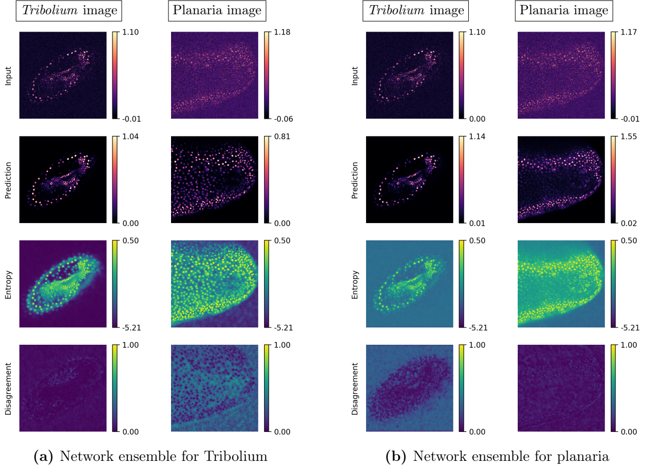
Supplementary Figure 28: Uncertainty read-outs for cross-applications of trained CARE networks. Two network ensembles applied to two input image stacks, yielding four different restorations. From top to bottom, we show slices of the input, the predicted restored image, the entropy of the ensemble, and the ensemble disagreement. We applied each network ensemble to an in-distribution (ID) image ( i.e. , an image similar to those the ensemble was trained on; first and last column) and an out-of-distribution (OD) image ( i.e. , an image dissimilar to the training data; two middle columns). Disagreement (last row) is often substantially higher when an ensemble is applied to an OD input image.
