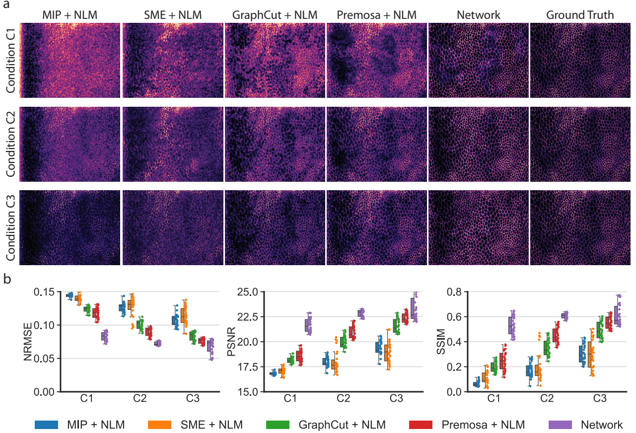
Supplementary Figure 11: Comparison of joint surface projection and denoising methods on developing Drosophila melanogaster wing epithelia. (a) Results on a single fly wing stack for 3 different SNR conditions. (b) Reconstruction accuracy measured on held out test set (comprising 26 volumetric stacks for each condition). (a,b) We compare the result of CARE (Network) with MIP (Maximum projection), SME (smooth 2D manifold extraction [7]), GraphCut (Minimum cost surface projection [8, 9]) and PreMosa (2D surface projection [1]), where we additionally applied NLM (Non-Local-Means [6]) on the output of all methods ( except ours ). Note that we tuned the NLM hyper-parameter for best results on the validation data, giving all baseline results an additional advantage.
