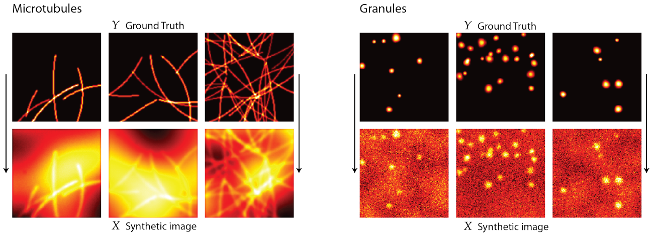
Supplementary Figure 21: Synthetically generated training data for microtubules and secretory granules. We first generate the ground-truth images (Y) by tracing tubular bundles of different sizes and length (left) or simulating granular regions (right) on pixel grids of size 128 \times 128 and pixel-size 0.08 \mu m . We then simulate the microscopy image (X) by adding low frequency perlin-noise resembling background fluorescence, convolving with the microscope PSF, and adding Gaussian and Poisson camera noise.
