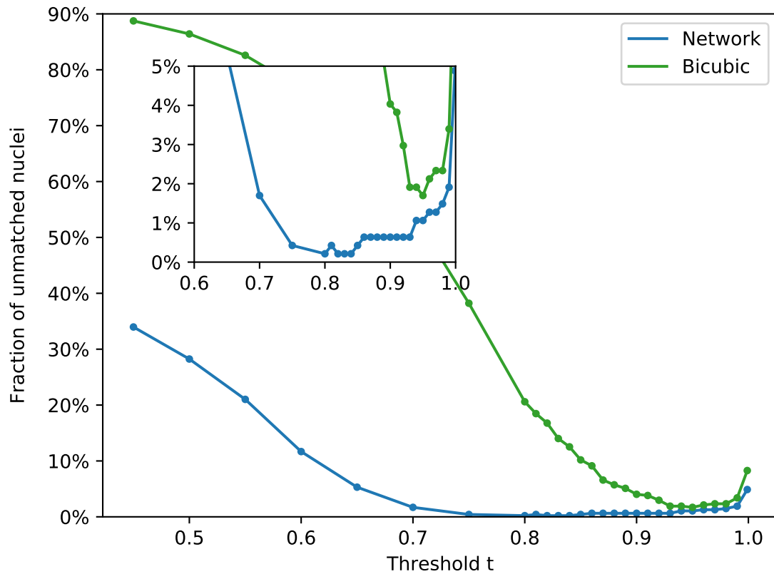
Supplementary Figure 18: Segmentation error of isotropically reconstructed and bicubically upsampled raw images of developing Drosophila melanogaster embryos. Shown is the fraction of unmatched nuclei (out of all 471 ground-truth nuclei) for varying levels of the threshold t . The lowest error is 0.2% (Network, t = 0.8 ), and 1.7% (Bicubic, t = 0.95 ). Note the wide region over which isotropically restored images produce a lower fraction of unmatched nuclei relative to bicubically upsampled images. For a visual comparison of the optimal segmentations see Supp. Fig. 17.
