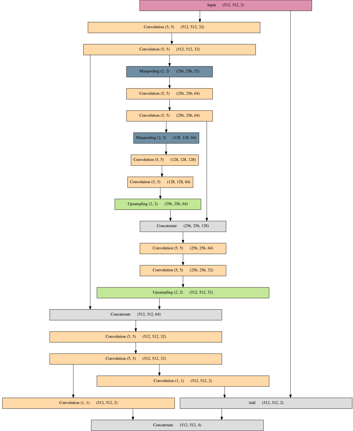
Supplementary Figure 13: Network architecture used for isotropic reconstruction. We use an architecture based on a 2D U-Net [4]. Shown is the architecture for a probabilistic model, that predicts a per-pixel distribution (parameterized by mean and scale) resulting in a 2-channel output. The mean is calculated as the sum of the input and the internal predictions ( residual addition layer near the end). For the non-probabilistic model only the mean is used as prediction.
