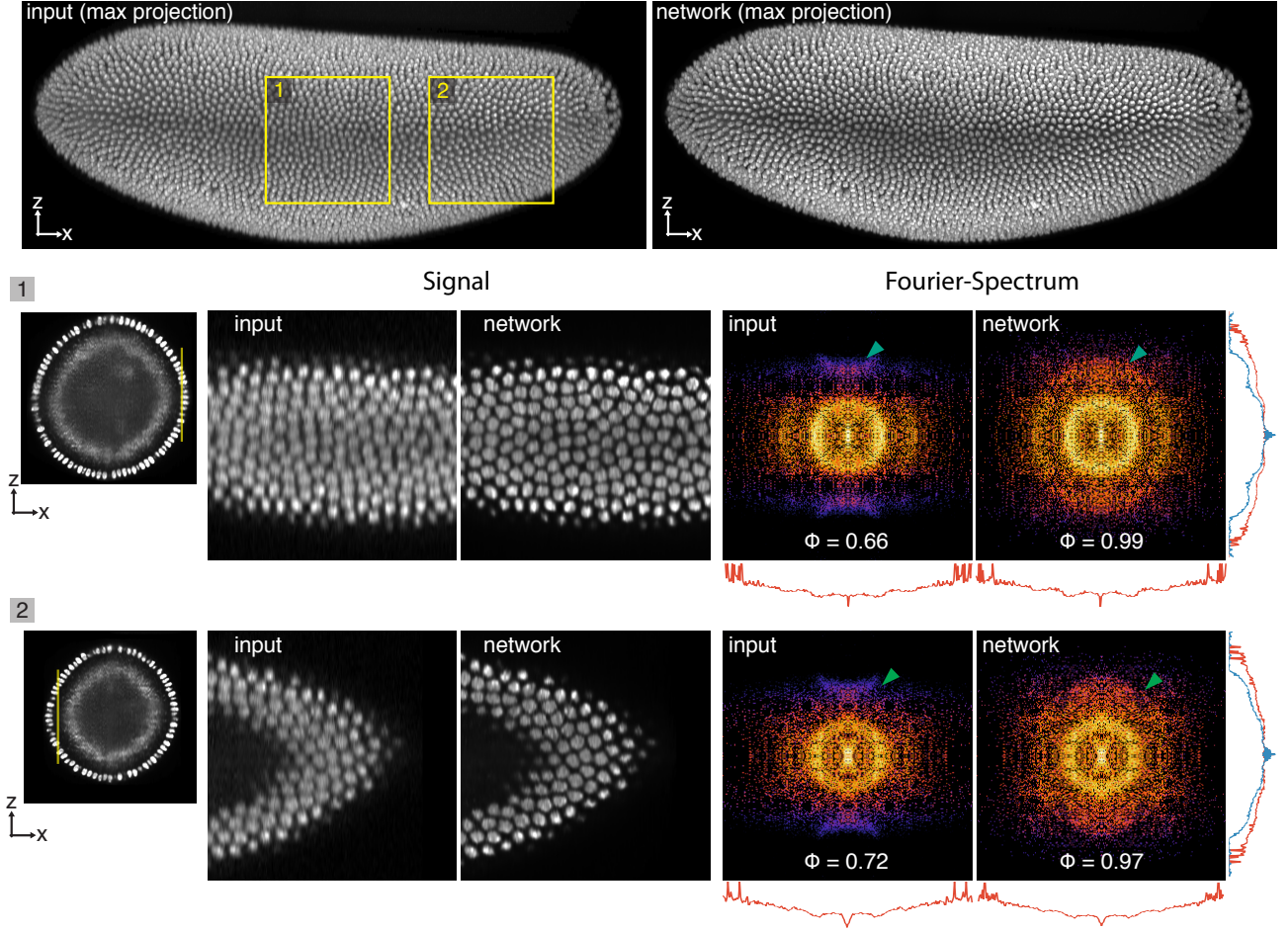
Supplementary Figure 16: Comparison and quantification of isotropic reconstruction of time-lapse acquisitions of developing Drosophila melanogaster embryos. Data was taken from [2] (5-fold under-sampled in z ). Axial resolution restoration as quantified by analyzing the ratio \Phi of axial vs. lateral spectral energy in Fourier space: \Phi = 0.66/0.72 (Input), \Phi = 0.99/0.97 (Network). Note that the missing axial information along the z -axis in Fourier-space is filled up by the restoration.
