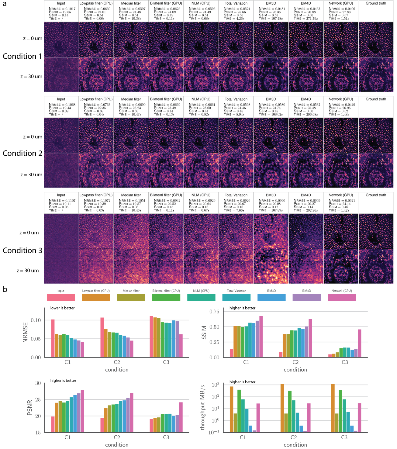
Supplementary Figure 5: Comparison of different denoising methods applied to low-SNR acquisition of Schmidtea mediterranea (planaria). Although impossible in practice, note that we tuned the hyper-parameters of all methods ( except our Network ) on the test image to yield their best possible results. (a) Output of compared methods for 3 different SNR conditions. For every condition two different slices ( z = 0\mu m and z = 30\mu m ) through the same volume of size (500 \times 500 \times 41) are shown. See Supp. Tab. 1 for details on all compared methods. All methods are 3D methods, apart from BM3D, which was applied plane-by-plane. (b) Error metrics and throughput for each method. We show NRMSE ( normalized mean squared error , lower is better), SSIM ( structural similarity index , higher is better), PSNR (higher is better) and throughput (input size/time, higher is better). Note that the slow runtime of BM3D and BM4D render both methods impractical for typical biological datasets ( \gg 1GB ).
