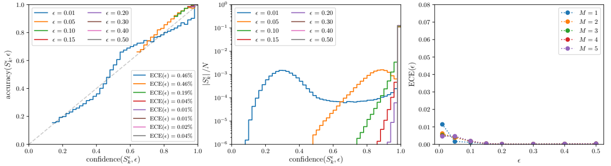
Supplementary Figure 27: Uncertainty evaluation of CARE network ensembles. (continued from Supp. Fig. 26).
