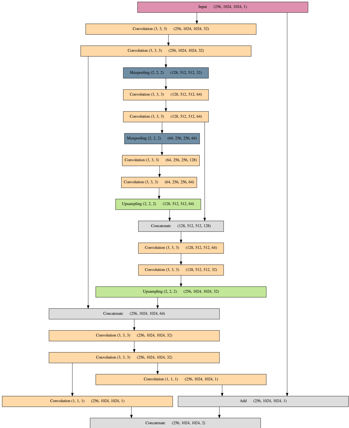
Supplementary Figure 1: Network architecture used for restoration of low-SNR stacks in 3D. We use an architecture based on a 3D U-Net [4]. Shown is the architecture for a probabilistic model, that predicts a per-pixel distribution (parameterized by mean and scale) resulting in a 2-channel output. The mean is calculated as the sum of the input and the internal predictions ( residual addition layer near the end). For the non-probabilistic model only the mean is used as prediction.
