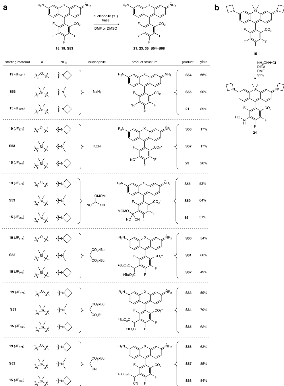
Scheme S4. (a) Nucleophilic substitution (S N Ar) reactions of 4,5,6,7-tetrafluororhodamines ( 15 , 19 , and S53 ) with various nucleophiles. (b) Synthesis of hydroxylamine 24 from JF 669 ( 15 ).
