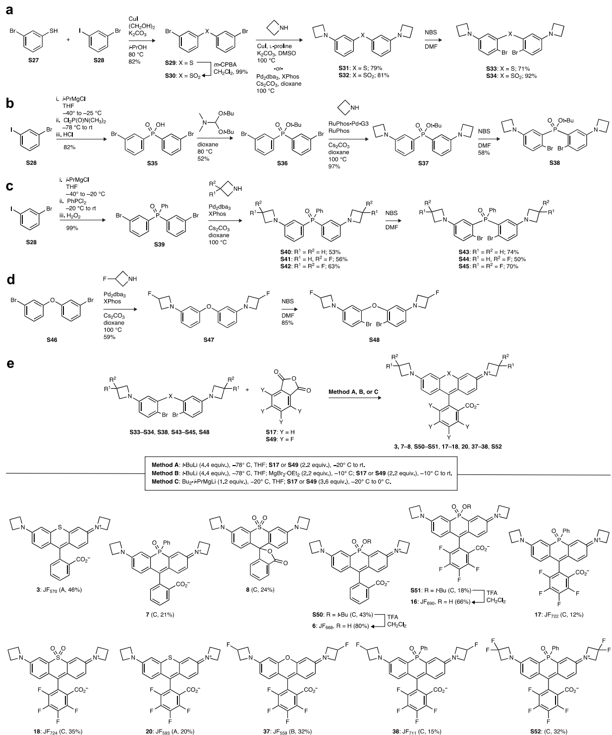
Scheme S3. (a) Synthesis of sulfide and sulfone dibromides S33 and S34 . (b) Synthesis of phosphinate dibromide S38 . (c) Synthesis of phosphine oxide dibromides S43–S45 . (d) Synthesis of ether dibromide S48 . (e) Synthesis of heteroatom-containing rhodamines 3 , 7–8 , S50–S51 , 17–18 , 20 , 37–38 , and S52 via metal–bromide exchange of the dibromides described in (a–d) and addition to anhydrides S17 or S49 ; TFA-mediated tert -butyl phosphinate deprotection of S50 and S51 yielded phosphinic acids 6 and 16 .
