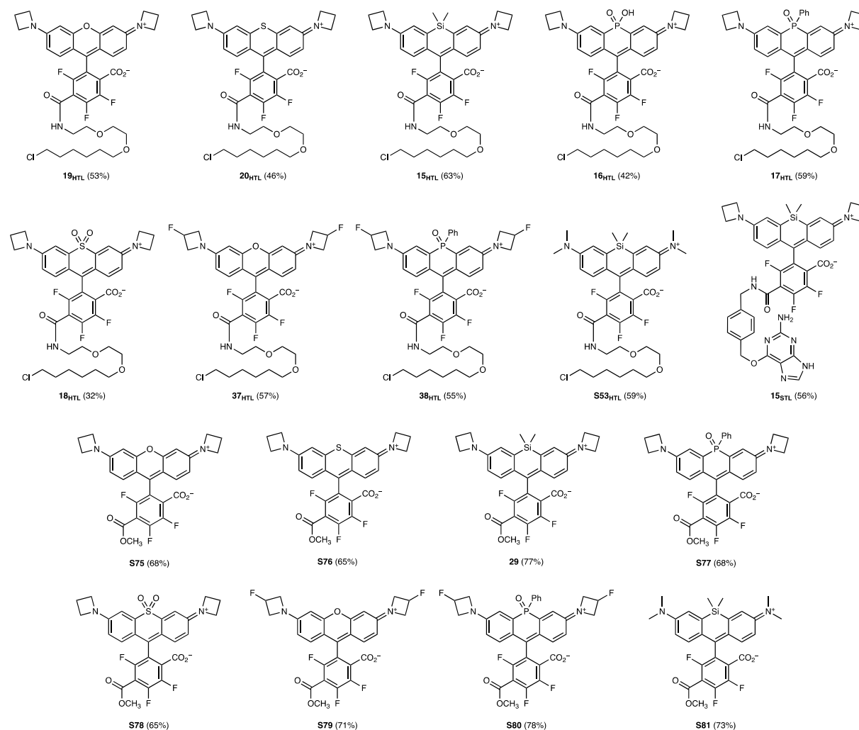
Scheme S5. Substitution of 4,5,6,7-tetrafluororhodamines with masked acyl cyanide (MAC) reagent 34 and subsequent derivatization to access HaloTag and SNAP-tag ligand labels and methyl ester analogs.
