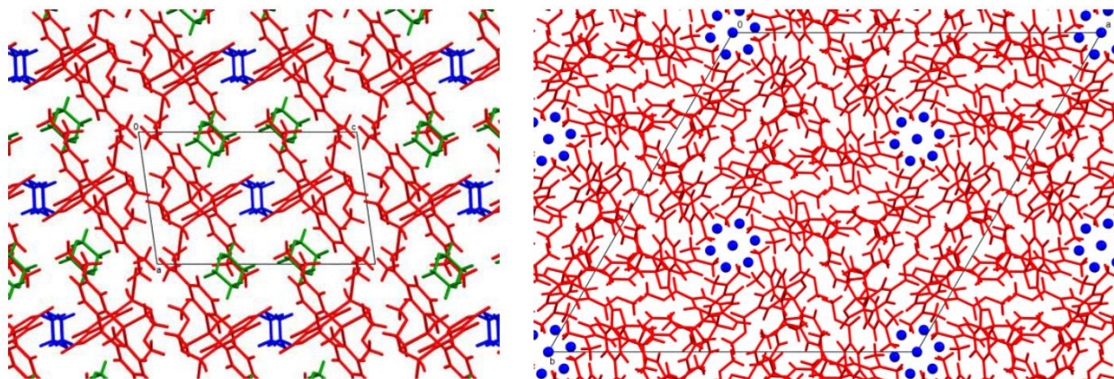
Figure S2. Packing along b axis in the crystal of S59 -1,4-dioxane solvate (left) and along c axis in the crystal of S81 -EtOAc solvate (right). In both images, S59 and S81 are shown in red while the solvent molecules are blue and green (left) and blue (right).
