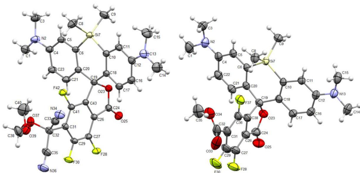
Figure S1. Molecular structure and atoms numbering scheme for S59 (left) and S81 (right); displacement ellipsoids at the 30% probability level.
