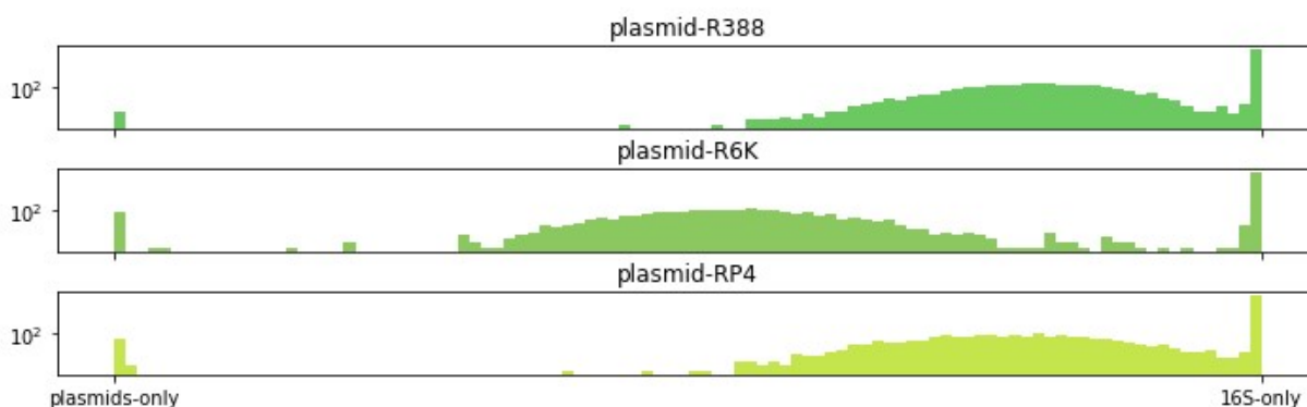
Figure SN2 Target primer balance plot for 3 plasmid targets in a DoTA-seq run showing relative amplification efficiency of each plasmid target compared to the 16S rRNA species marker gene. Y-axis is on a log scale although it looks very similar on a linear scale. X-axis represents the fraction of reads for each cell that maps to the 16S rRNA gene on a linear scale. Therefore, a distribution skewed towards 16S-only, such as for the target plasmid RP4 or R388, represents a lower relative capture efficiency target compared to the 16S species marker gene.
