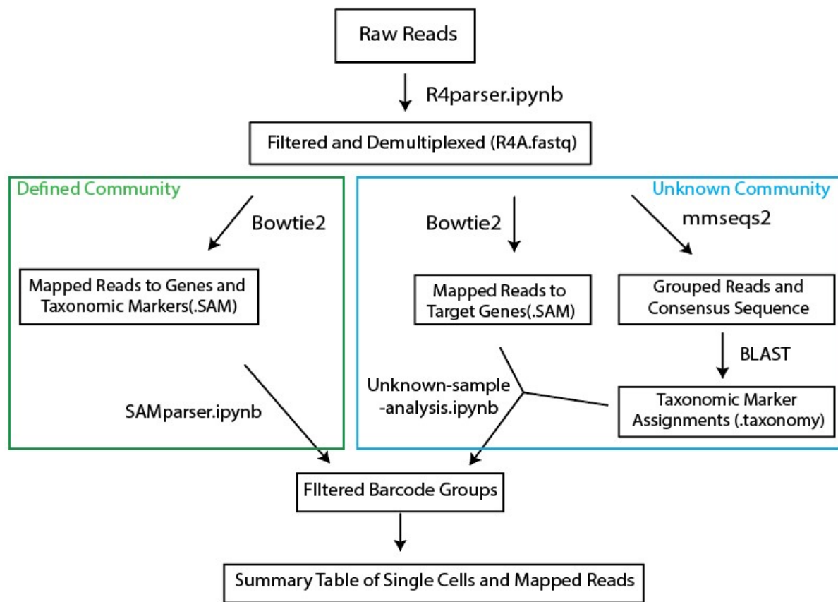
Supplementary Figure 1. Sequence analysis and filtering pipeline for DoTA-seq. Boxed text represent data and arrows represent scripts or programs used to process the data. Green box contains analysis specific to communities of known composition, and blue box contains analysis specific to communities of unknown composition. Raw reads obtained from the sequencer are processed in Python (R4parser.ipynb) to remove low quality barcodes and associate the droplet barcodes with the amplicon reads. The resulting reads are processed differently depending on the source sample material. For defined microbial communities, reads are mapped to a reference containing all target genes and taxonomic marker genes using Bowtie2, obtaining a SAM file. This SAM file is analyzed using Python (SAMparser.ipynb) to filter droplet barcodes based on evidence of cross-contamination and minimum numbers of reads (more details in the Github README file). For reads from unknown (i.e. naturally derived) communities, all reads are first mapped to a reference containing the non-taxonomic marker target genes using Bowtie2. For taxonomic classification, all reads are first clustered by pairwise similarity using mmseqs2, then the consensus sequence for each grouped cluster is used to search a BLAST database of taxonomic markers (such as 16S rRNA database). These results are combined with the Bowtie2 results then filtered based on markers of cross-contamination and minimum numbers of reads using Python (Unknown-sample-analysis.ipynb). More details are available in the README file on the Github page.
