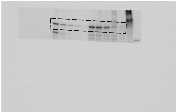
Anti-Rev3 blot
