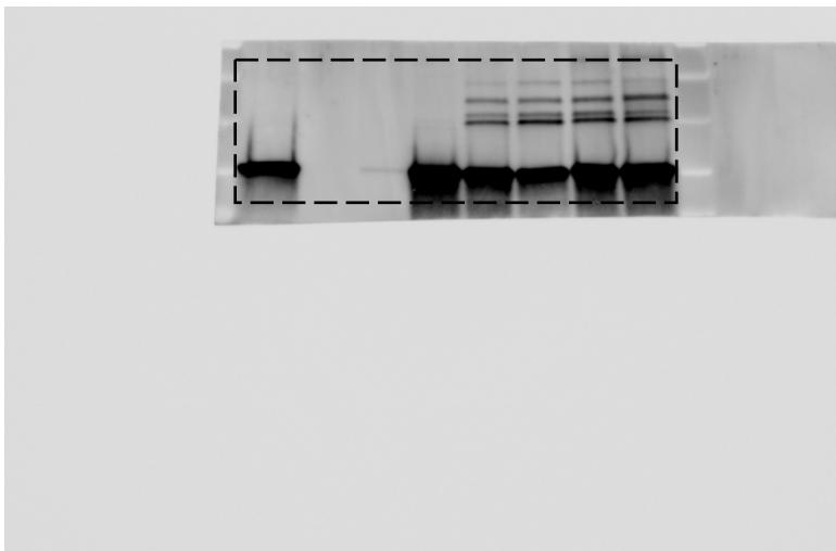
Anti-Pcna
