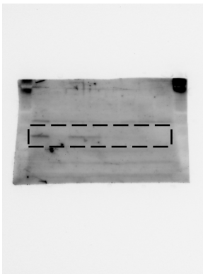
Anti-Rev7 blot
