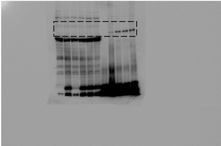
Anti-FancA blot
