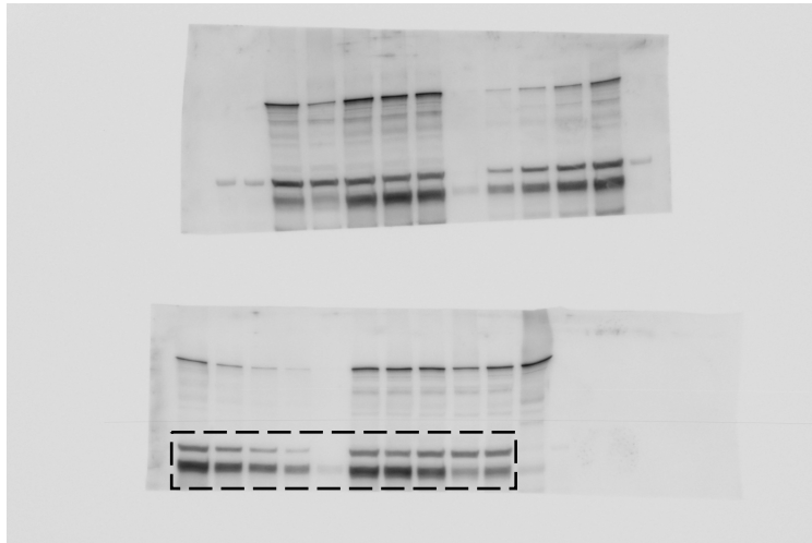
Anti-Rev1 blot
