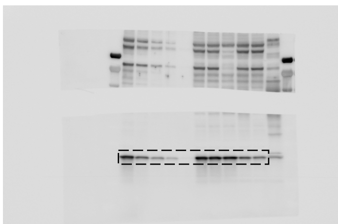
Anti-Rev7
