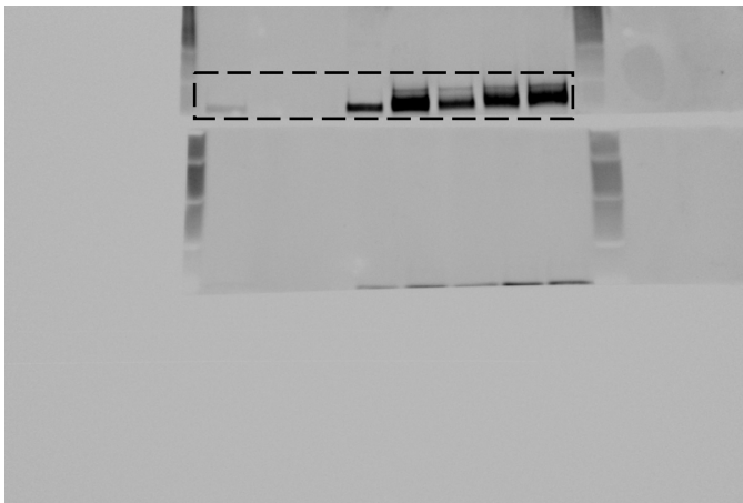
Anti-Pcna
