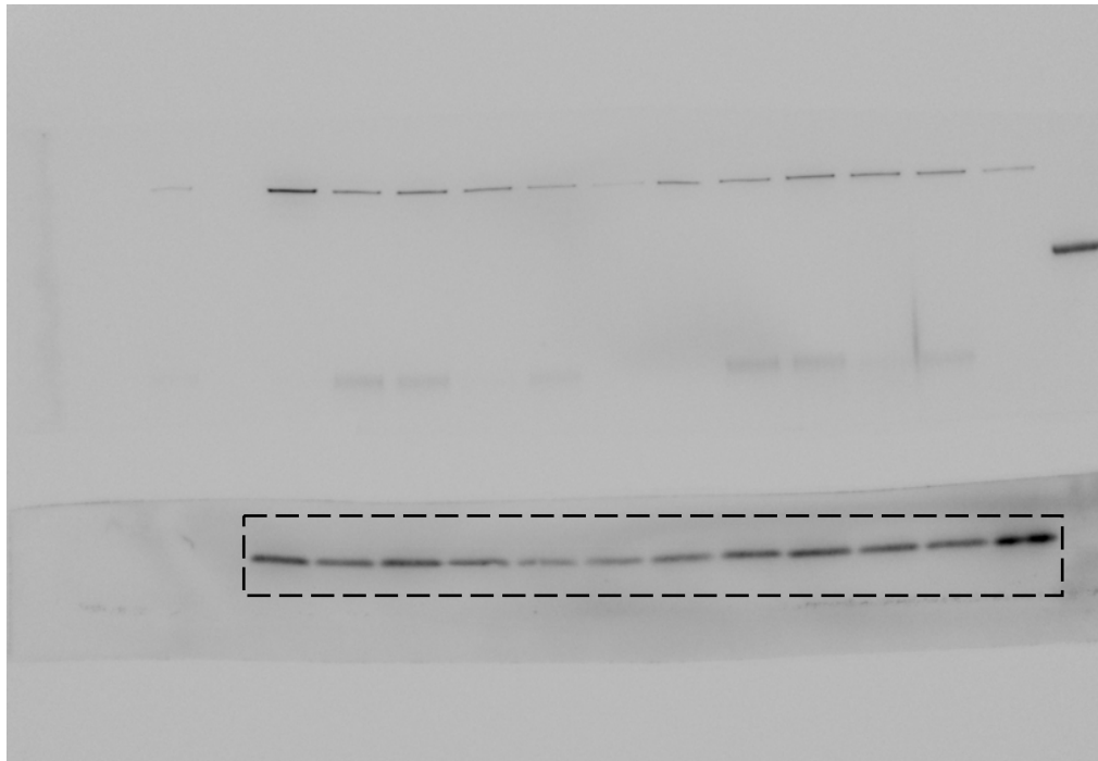
Anti-H3
