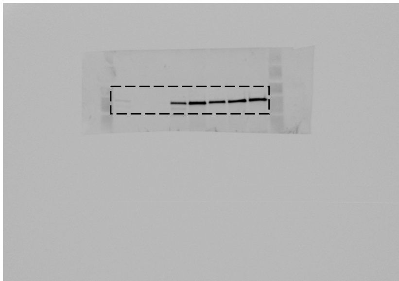
Anti-Scai blot
