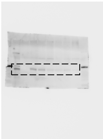
Anti-Rev1 blot
