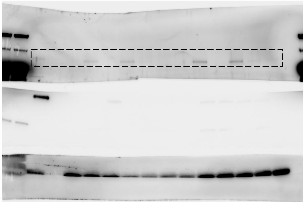
Anti-Pol kappa
