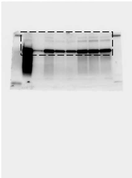
Anti-Pcna blot
