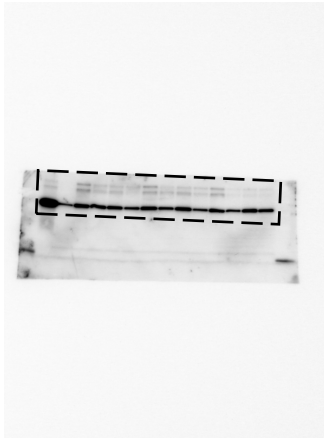
Anti-Pcna blot
