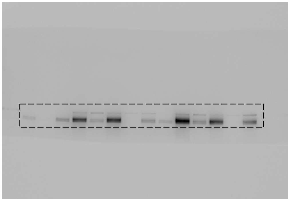
Anti-Rev1 blot
