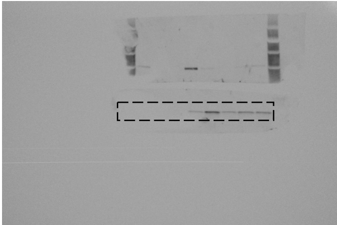
Anti-Rev1 blot
