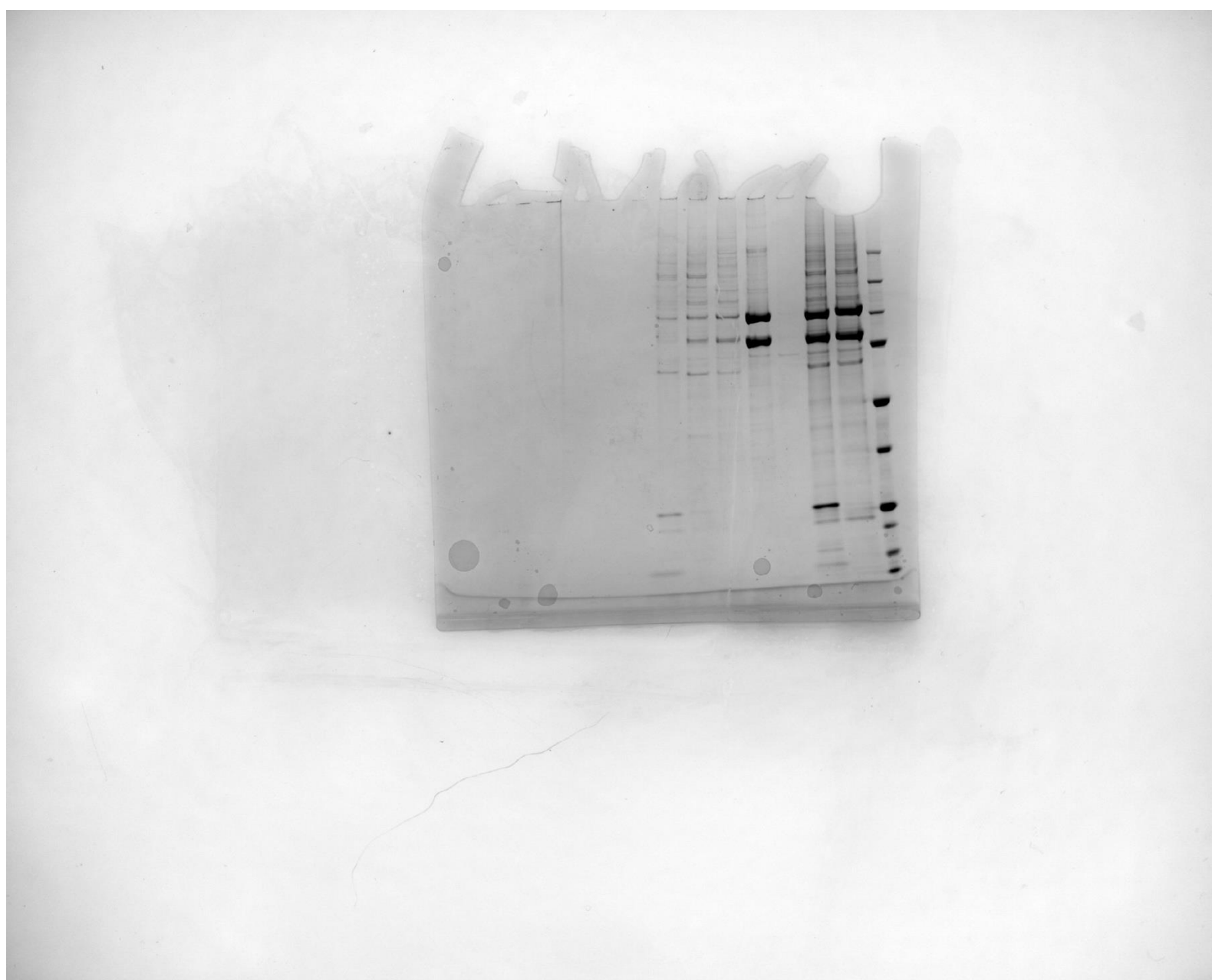
Sec23-Sec24 purification gel (Extended data Fig 1A)
