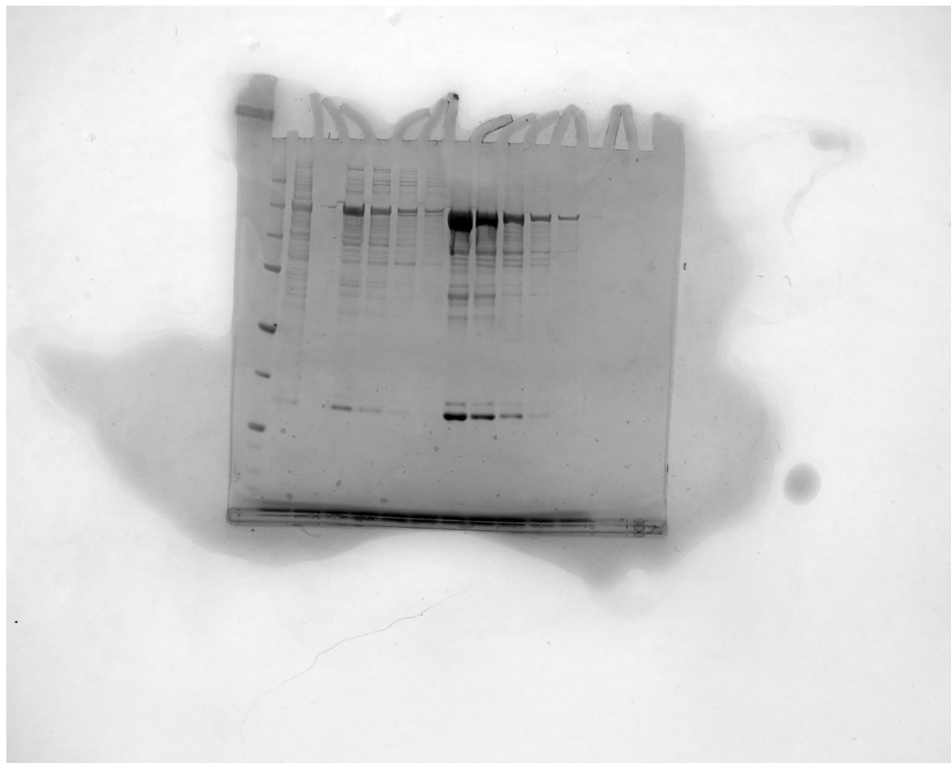
Sec13-Sec31 purification gel (Extended data Fig 1A)
