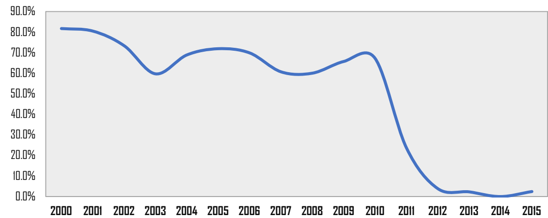
Fig.1 Capacity factor variation (Ratio) for nuclear power plant in Japan from 2000 to 2015
