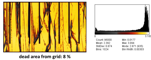
Supplementary figure 1. Laser-beam induced current measurement of the back-textured IBC solar cell.
