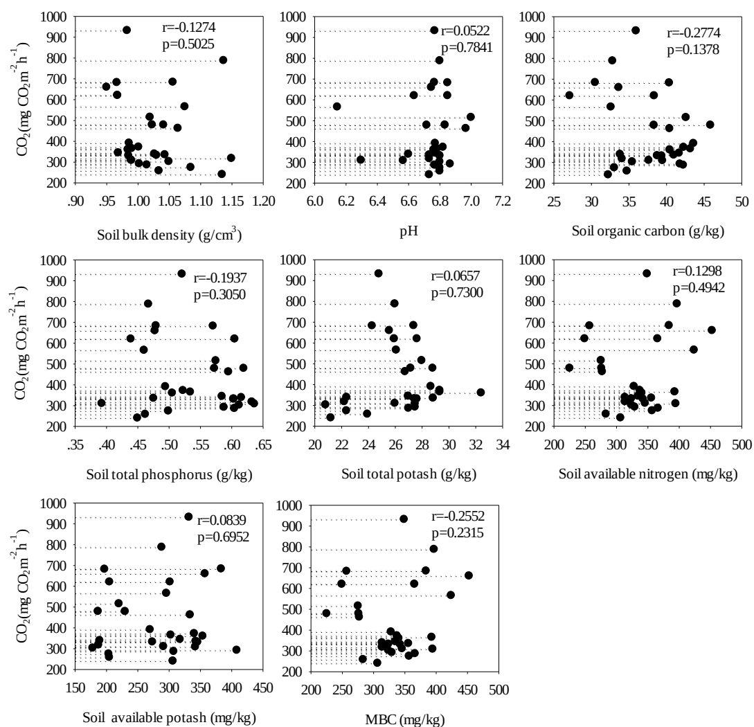
Supplementary Fig. 1. Relationships between the mean ecosystem CO 2 fluxes and soil other factors (soil bulk density, pH, soil organic carbon, soil total phosphorus, soil total potash , soil available nitrogen, soil available potash and MBC) from all plots across five years.
