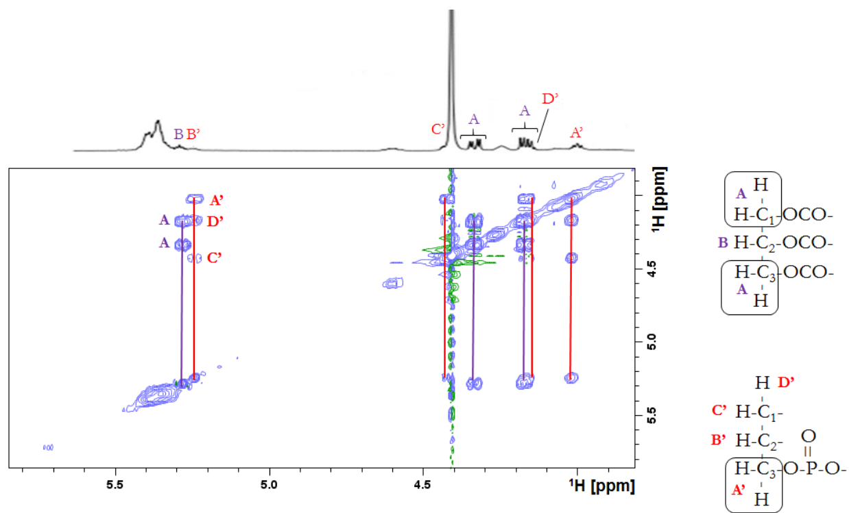
Figure S2. The ^1\text{H} - ^1\text{H} TOCSY spectrum of MO patients' serum determining the position of TG and PL protons. TG - violet lines; PL - red lines.
