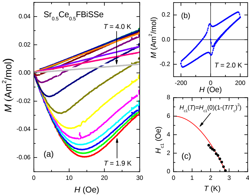
Fig. S7 (a) Low field magnetization of \text{Sr}_{0.5}\text{Ce}_{0.5}\text{FBiSse} at temperatures of 1.9 - 3.2 K in steps of 0.1 K, and at 3.4, 3.5, 3.75 and 4.0 K. (b) Superposed ferromagnetic and superconducting magnetization loop at 2.0 K. (c) Lower critical field H_{c1}(T) (solid symbols). The red line represents the standard quadratic temperature variation of H_{c1} .
