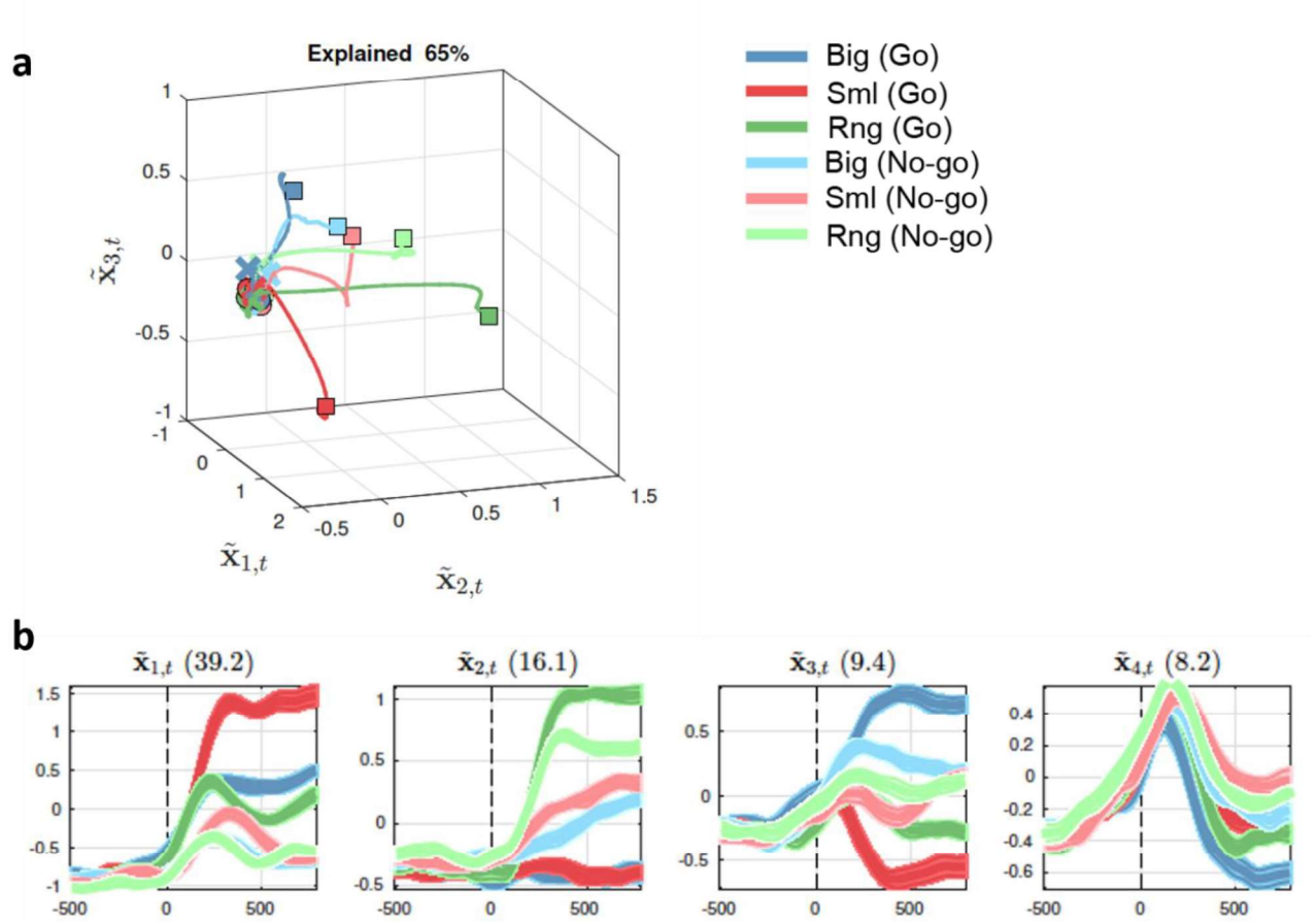
Figure S1. Neural space analysis with aggregated data from M1 and M2 - pragmatic task (PT). (a) Trajectories in the 3D "neural space" formed by the first three principal components of PCA, during the pragmatic task (PT). The neural trajectories span the interval [-500, 800] , with zero being the target onset, and each bin representing the average of 200 ms. Circles mark the beginning of the neural trajectories, crosses mark target onset, and squares mark the end of the neural trajectories. (b): Trajectories in the 1D space of the first 4 components of PCA (one panel for each component). Mean (coloured line) and variance (coloured shades) are shown.
