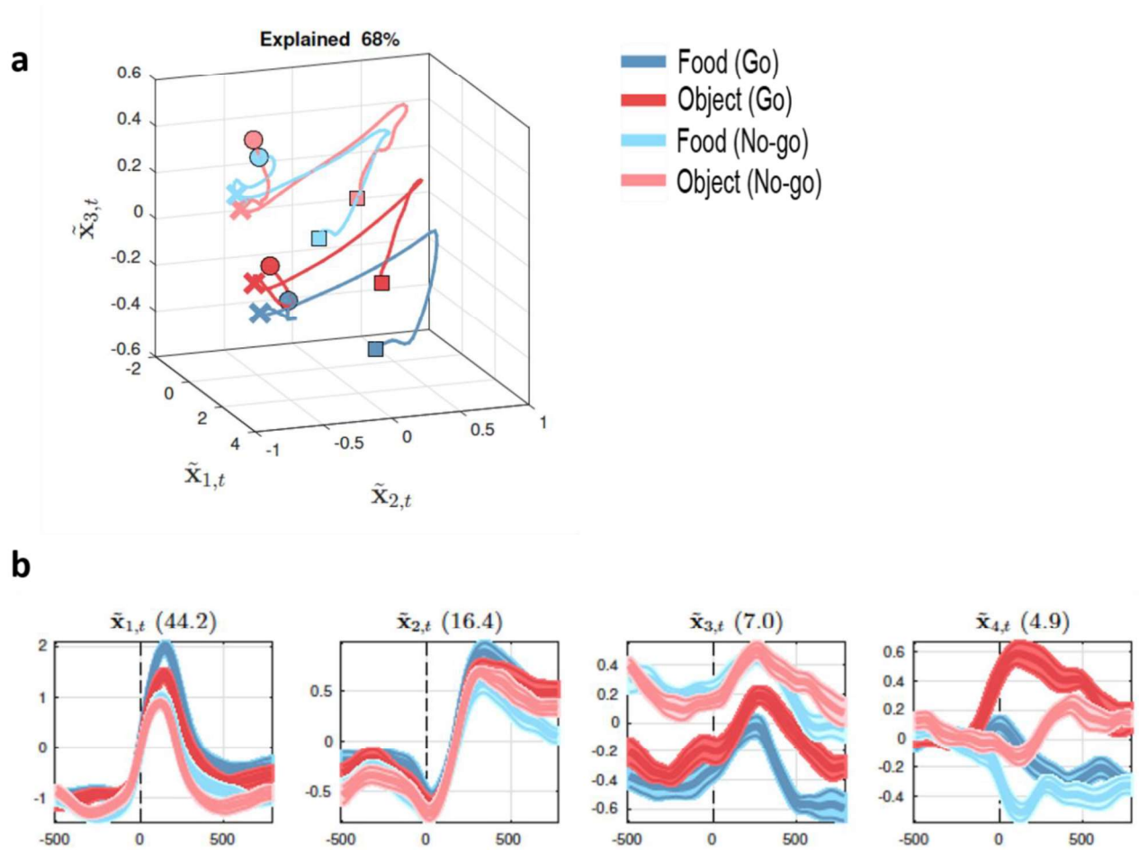
Figure S3. Neural space analysis with aggregated data from M3 and M4 - semantic task (ST). (a) Trajectories in the 3D "neural space" formed by the first three principal components of PCA, during the pragmatic task (PT). The neural trajectories span the interval [-500, 800] , with zero being the target onset, and each bin representing the average of 200 ms. Circles mark the beginning of the neural trajectories, crosses mark target onset, and squares mark the end of the neural trajectories. (b) Trajectories in the 1D space of the first 4 components of PCA (one panel for each component). Mean (coloured line) and variance (coloured shades) are shown.
