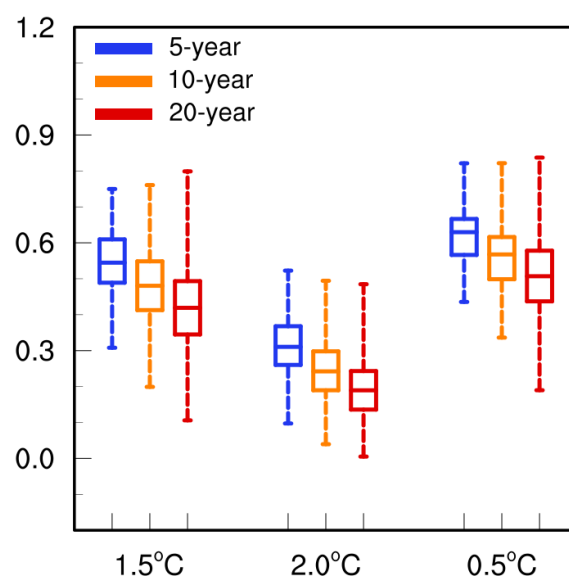
Figure S2. As in Fig. S1, but for 5-, 10- and 20-year TNn.
