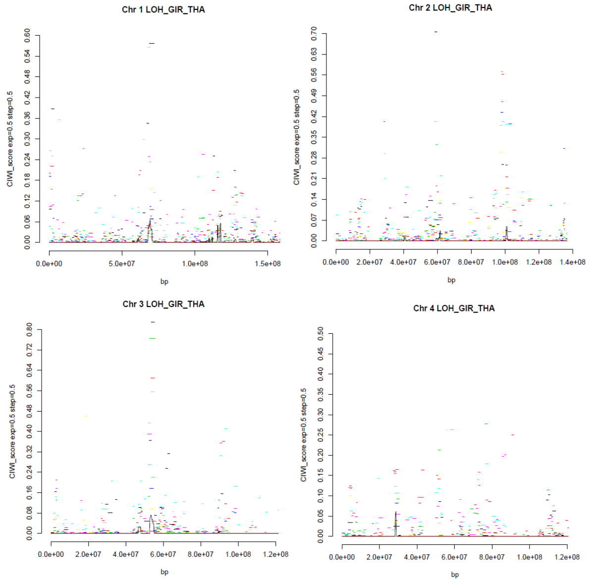
Figure S5. CIWI results for 29 chromosomes. Chianina was used as target population, Hereford, Fleckvieh and Brown Swiss as taurine references, and Lohani, Gir and Tharparkar as indicine references. The solid black line represents the score assigned to the CIWI of indicine ancestry. See Table 1 for population labels.
