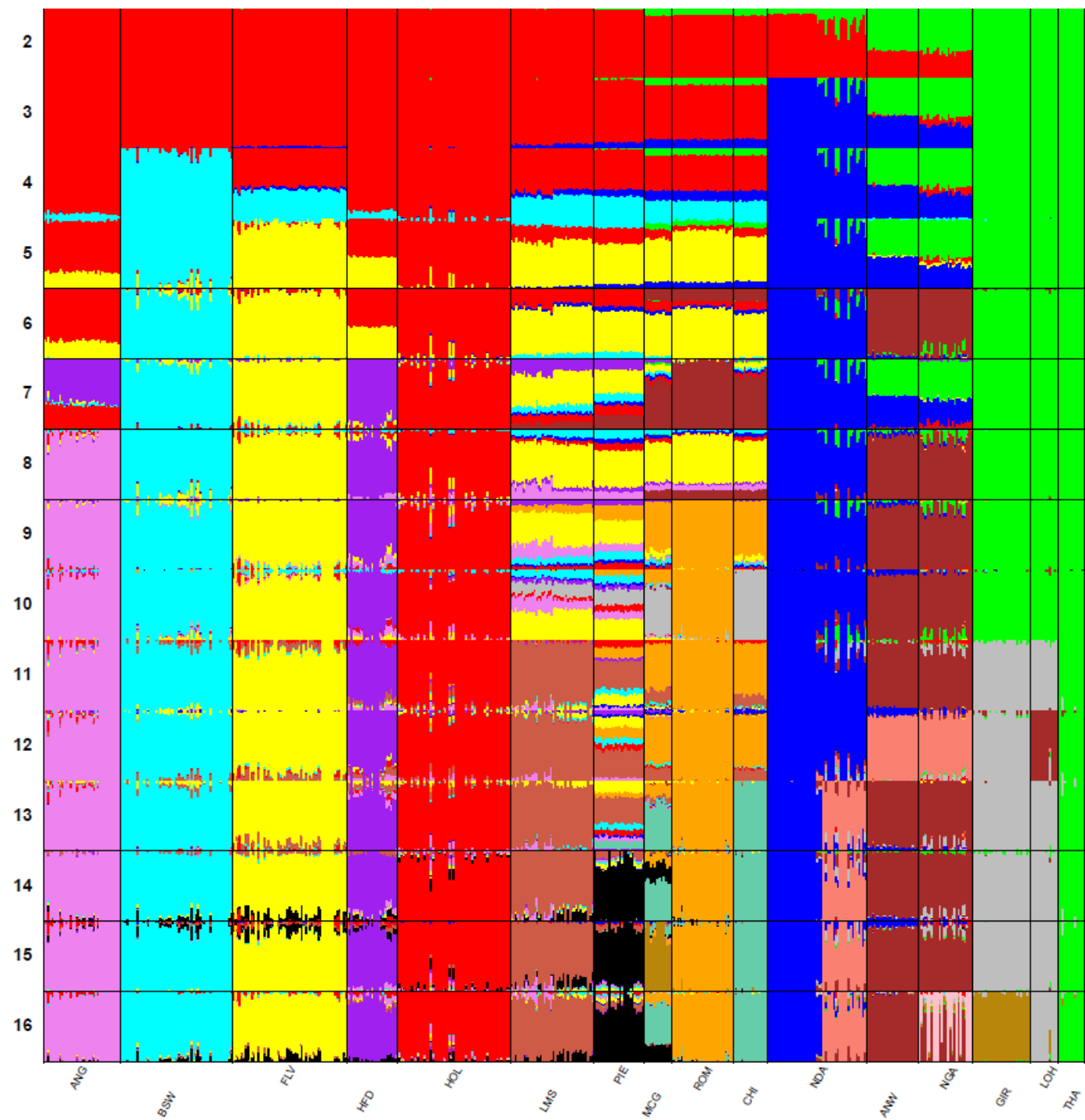
Figure S1a. Admixture plot of 16 cattle breeds based on 647,132 SNPs from the BovineHD SNPChip. Breed labels are available in Table 1.
