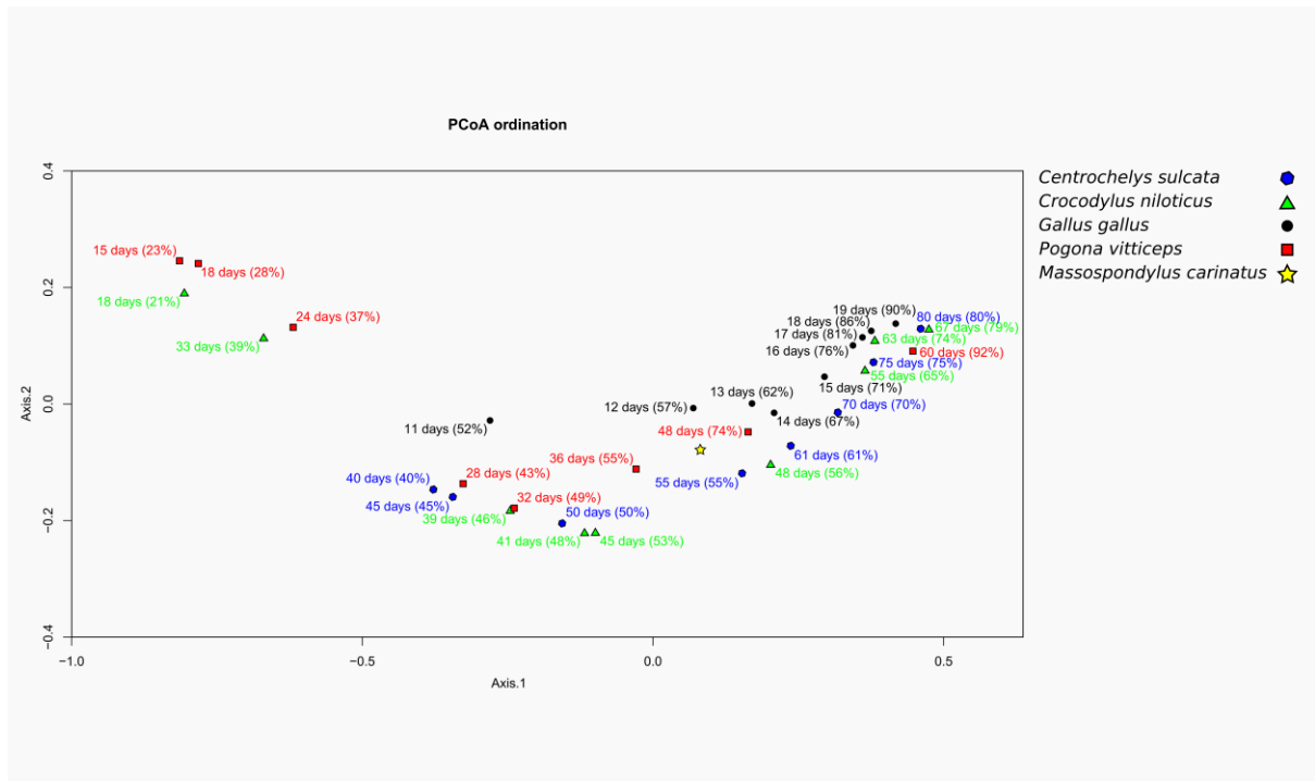
Figure S8. PCoA ordination plot.
