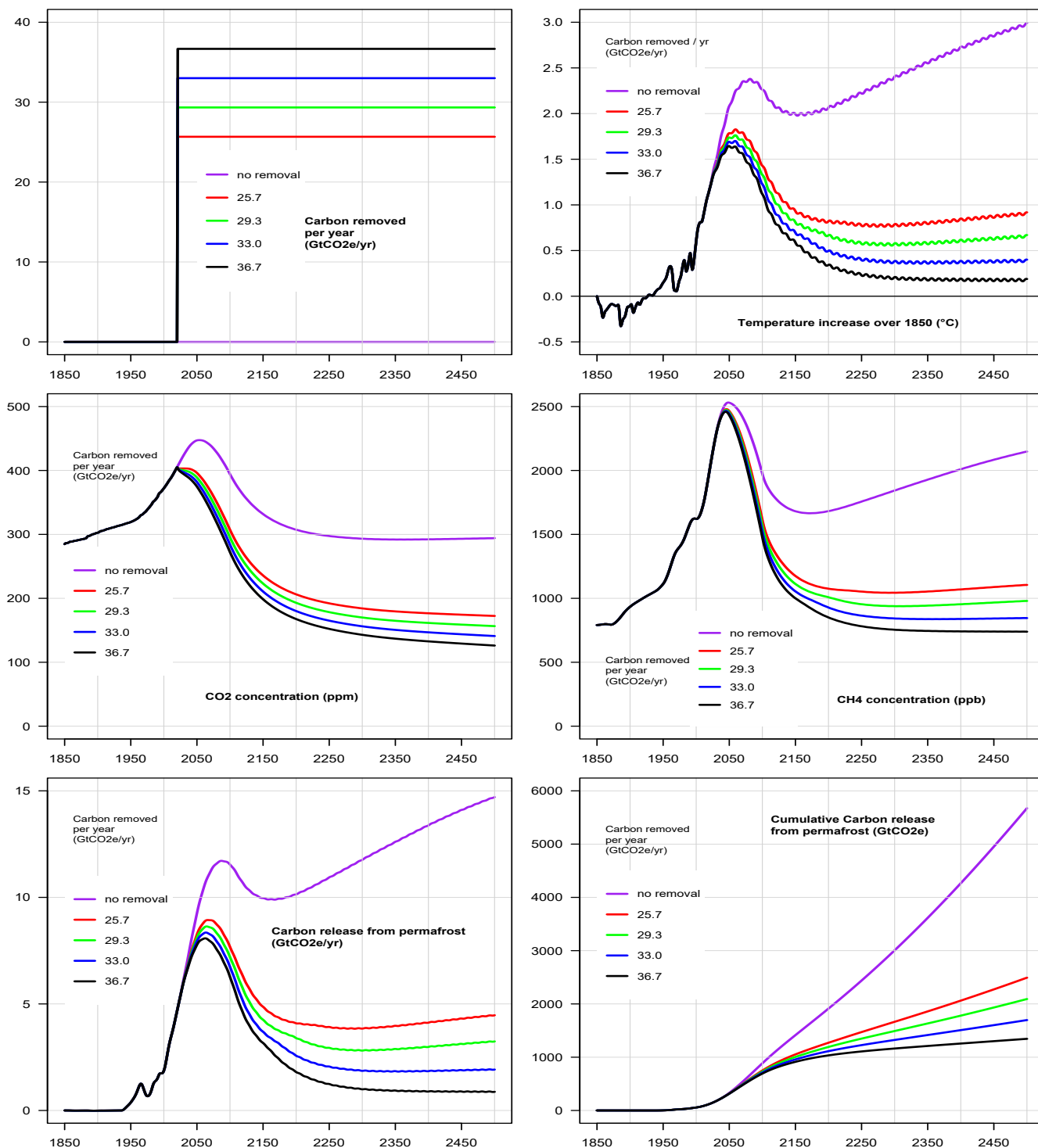
Supplement Figure 14 b (carbon in GtCO 2 e)
