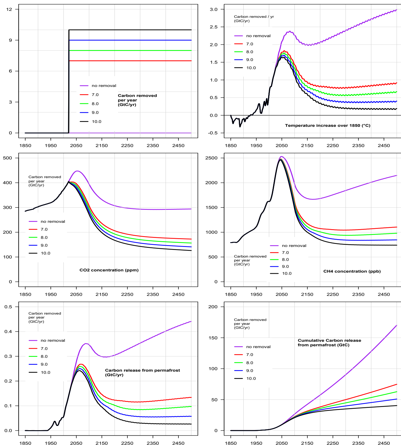
Supplement Figure 14 a (carbon in GtC)
