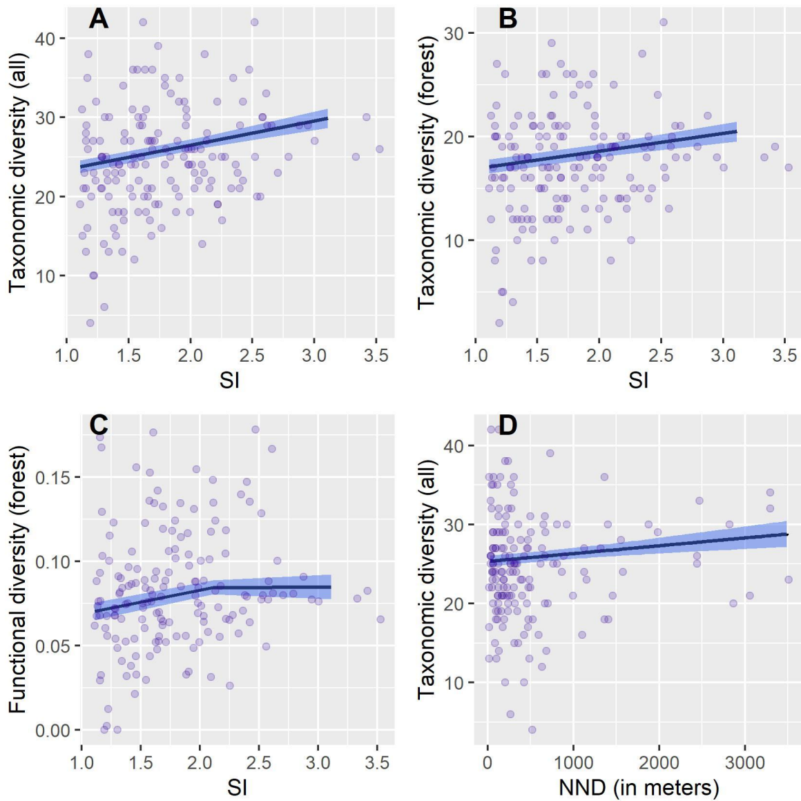
Figure S1. Response curves, derived from General Additive Modelling, showing the relationship between taxonomic and functional diversity (calculated for all of the bird species and forest specialist group) and forest patch shape index (SI) and nearest neighbour distance (NND).
