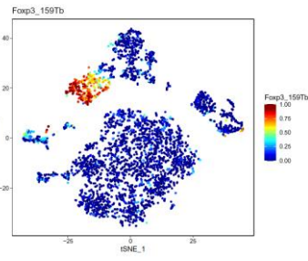
FOXP3_159Tb
