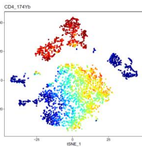
CD4_174Yb
