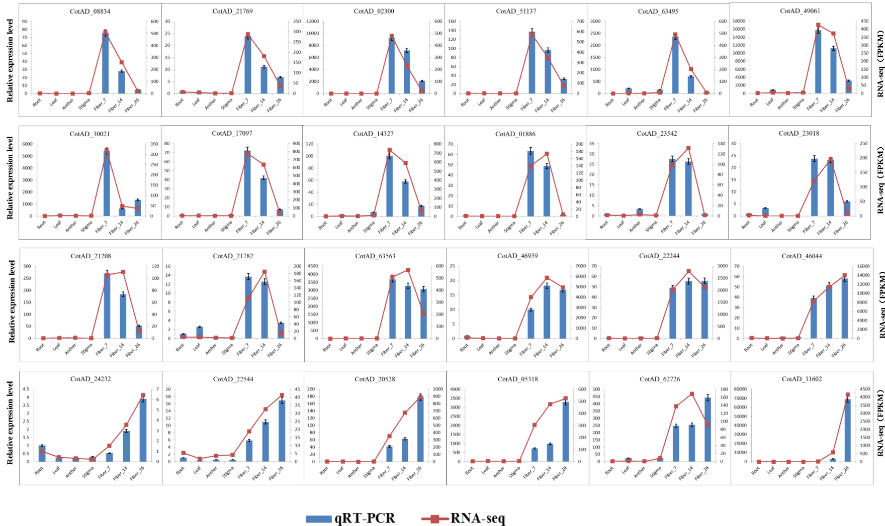
Figure S5. Validation of RNA-seq data by qRT-PCR.
