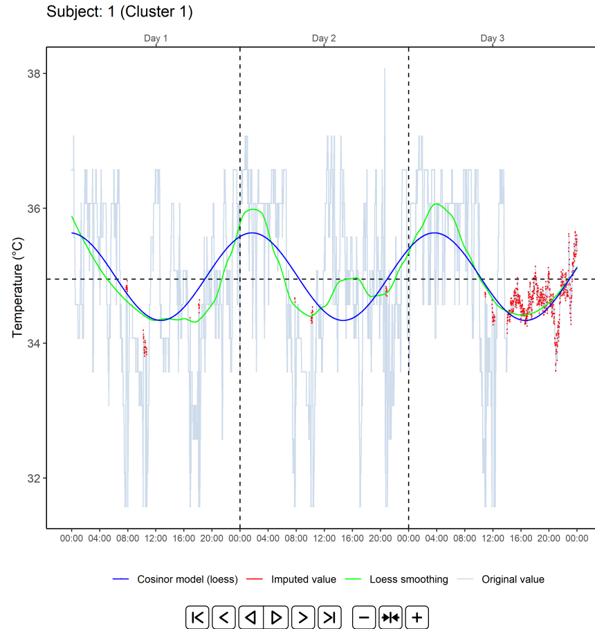
Supplement Figure S1: Individual observations, loess smoothing and predicted values of cosinor model based on the smoothed data. Horizontal dotted line equals average observed temperature over three days. Vertical lines indicate change of calendar day. Red dots indicate imputed missing values which are imputed using the regularised iterative PCA algorithm (Josse and Husson, 2013). Use control buttons to review all figures in the animation. Cluster membership is mentioned in the title and "Not included" indicates that subject is not included in the final analysis due to a missing values in sleep outcome variables or is rejected based on sensitivity analysis.
