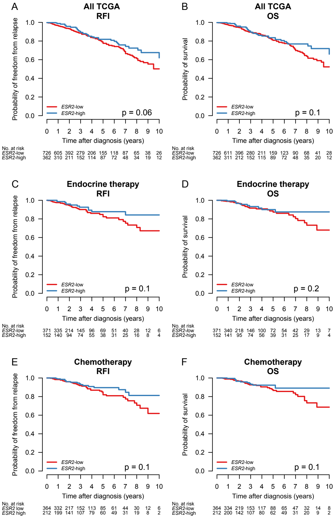
Supplementary Figure S1: ESR2 expression and association to overall survival (OS) and relapse-free interval (RFI) in the full TCGA cohort ( A , B ), the endocrine-treated sub-group ( C , D ) and the chemotherapy-treated subgroup ( E , F ).
