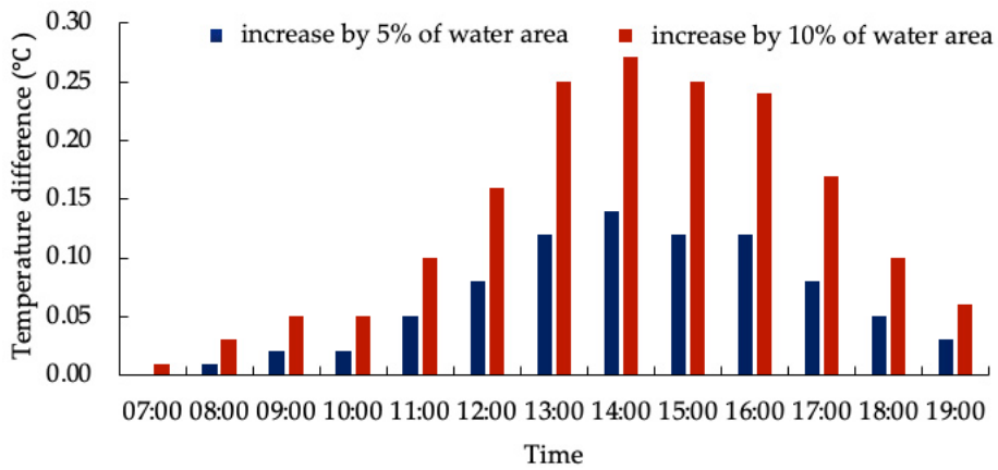
Figure 5 Differences in temperature in different simulated areas of annular water
