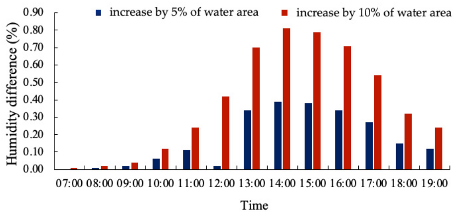
Figure 6 Differences in humidity in different simulated areas of annular water
