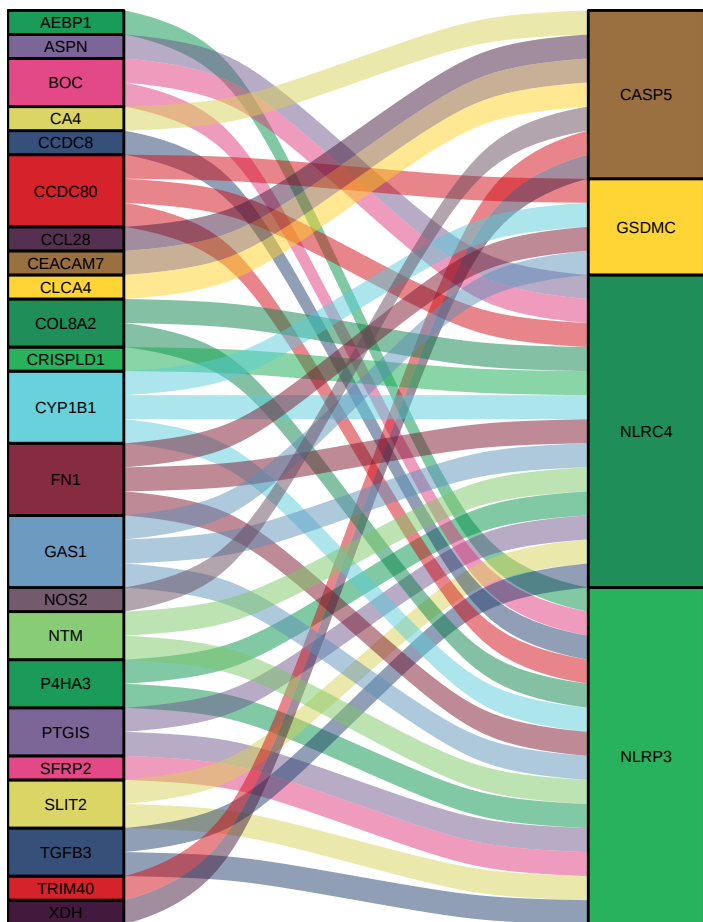
Figure S1: The correlation between DEGs and pyroptosis-related genes
