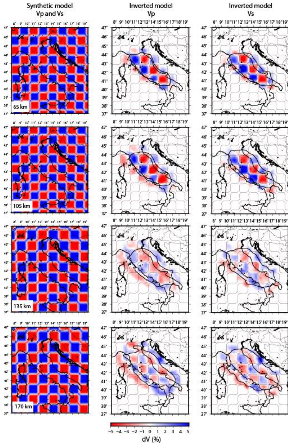
Figure SOM1: Results of the checkerboard test for Vp and Vs models . The reproduction of synthetic anomalies is good in the model, the black lines encircle the resolved areas as defined by the spread function analysis.
