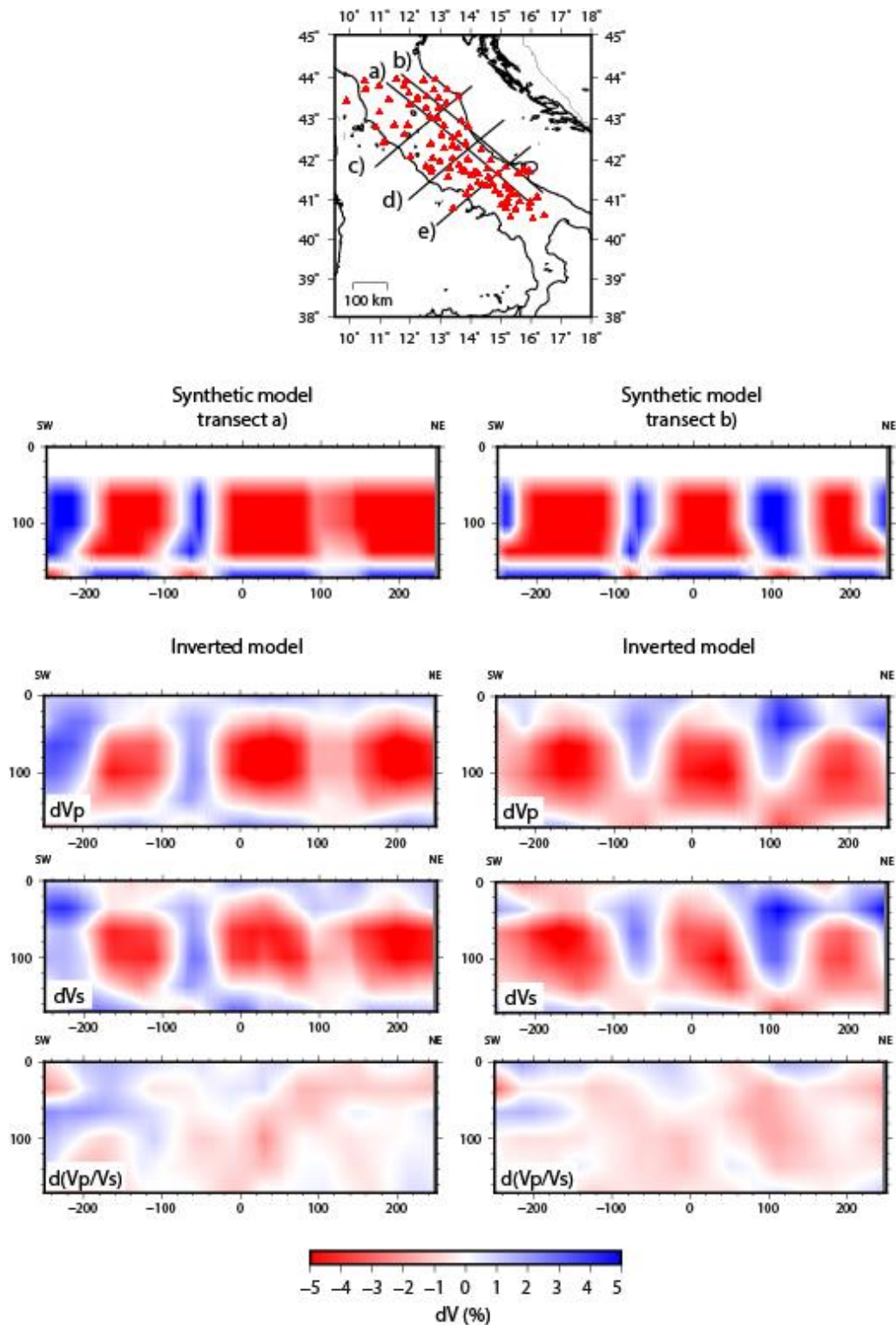
Figure SOM2: Results of the checkerboard test for Vp and Vs models in vertical sections, along the profiles reported in the manuscript.
