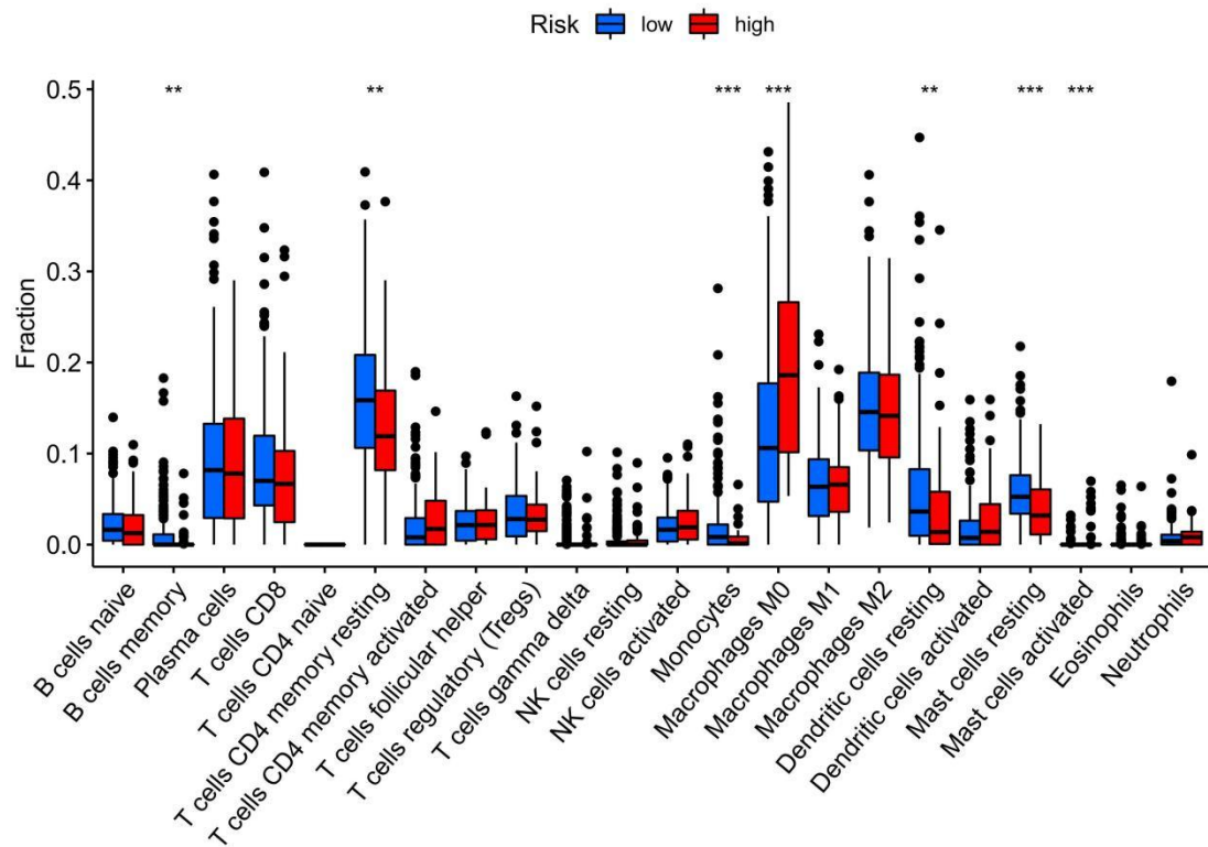
Supplementary Figure 5. The relative contents of 22 immune cell infiltration calculated by CIBERSORT method using R software. * p -value < 0.05, ** p -value < 0.01, *** p -value < 0.001.
