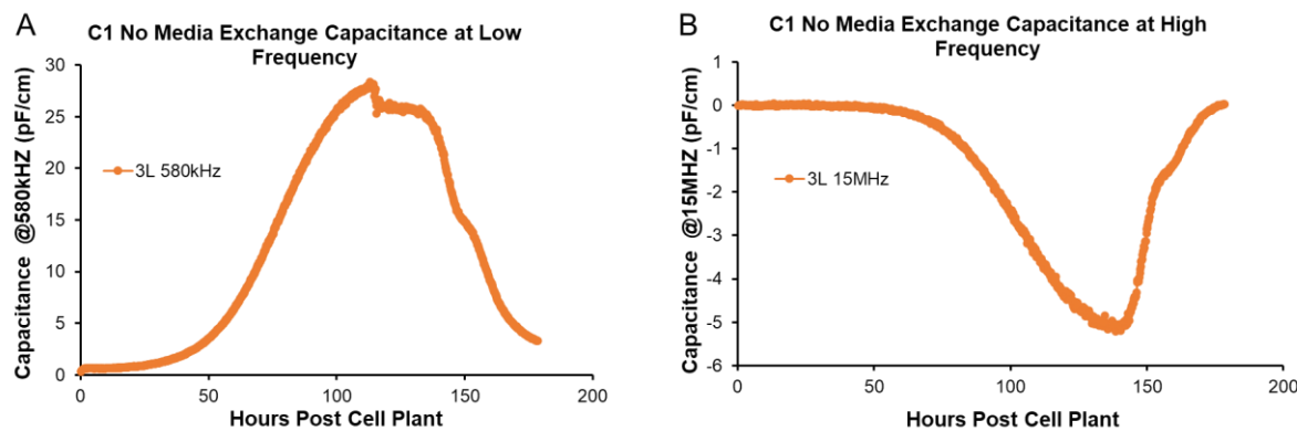
Figure S1. Biomass time profile of VSV-vector vaccine (C1) in a 3L bioreactor without the media exchange unit operation preformed in hours post cell plant measured at (A) 580kHz. and (B) high frequency (15MHz).
