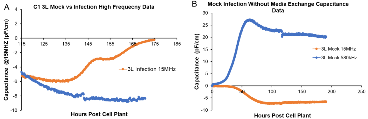
Figure S3. (A) Comparison of capacitance profiles at 15MHz for VSV-vector vaccine (C1) in a 3L bioreactor with a mock infected 3L bioreactor (blue) processed in a similar manner. (B) Biomass time profile of mock infected 3L bioreactor without the media exchange unit operation at 580kHz and 15MHz.
