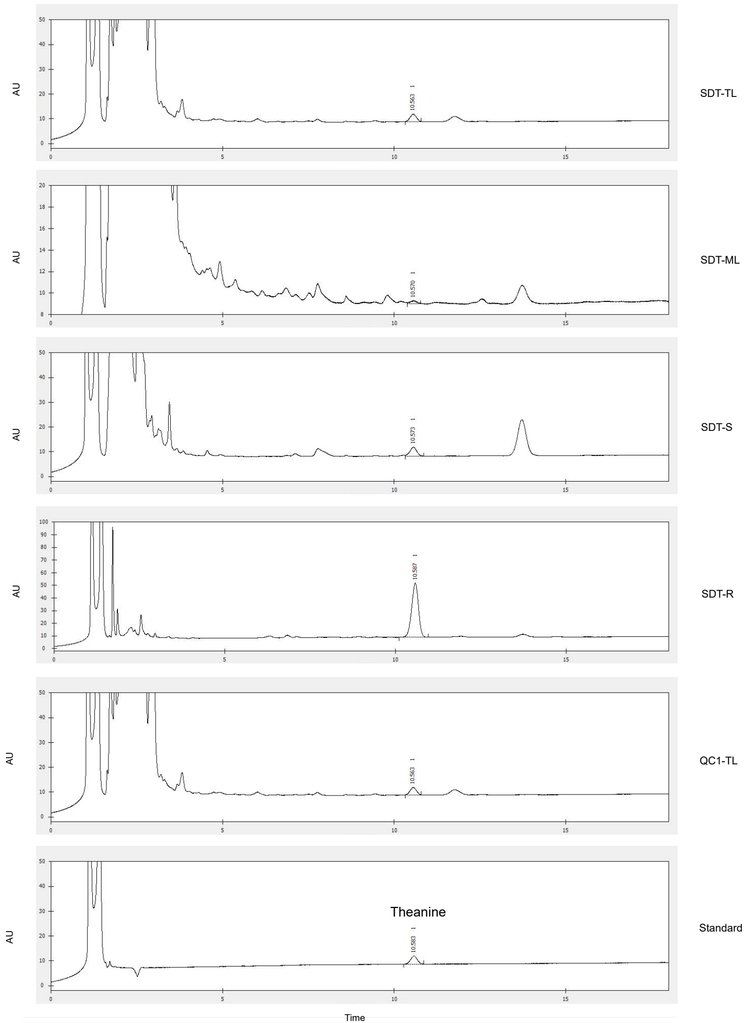
Figure S2. HPLC chromatogram of catechins, purine alkaloids EC and theanine in QC1 and SDT.
