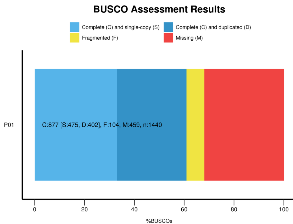
Figure S3. BUSCO assessment of assembled full-length transcriptome.
