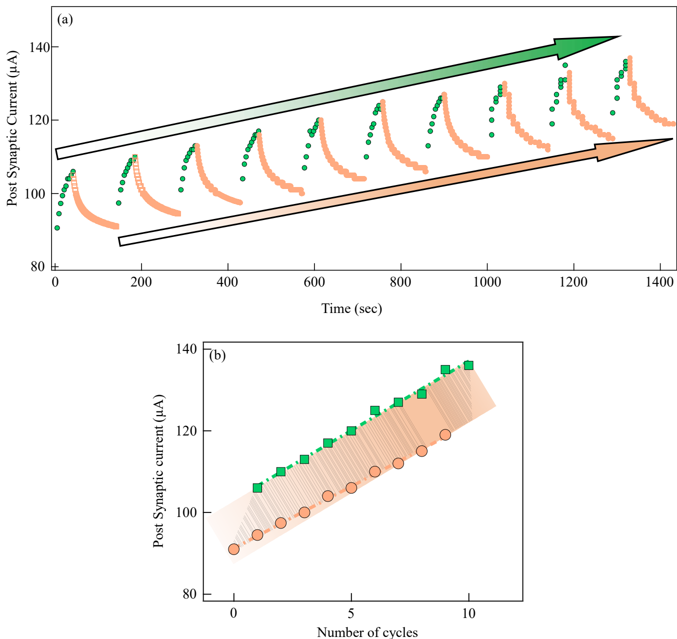
Figure S7 : Emulating the learning – forgetting – relearning curves for NiO nanoparticle based synapse. A series of 10 cycle operation increases the post synaptic current from 90.6 \mu\text{A} to 119 \mu\text{A} . For each Learning curve, 10 pulse ( ) are applied and then the PSC is monitored with time. A linear increase in the PSC can be useful for memory function. (b) The PSC after pulsing (green) and PSC after monitoring for 2 min ( orange). Both vary linearly with number of cycles showing an efficient biological synapse using NiO nanoparticles.
