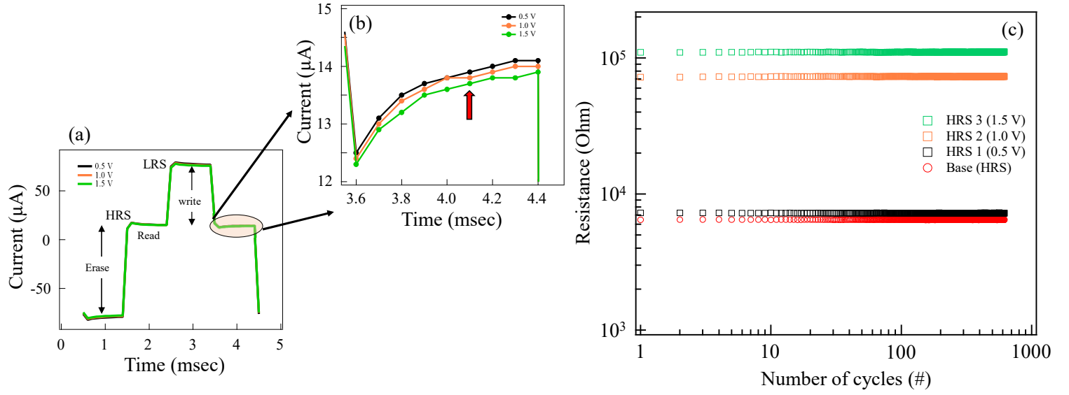
Figure S4: The multi-conduction state operation of the artificial synapse. Read – Write – Erase voltage pulses are applied to the synapse and the post synaptic current is monitored. (a) Single pulse sequence of erase – read – write – read – erase. The erase pulse and write pulses are varied and the post-synaptic current (PSC) is monitored. The device is taken to a low resistance state (LRS) from a previously maintained high-resistance state (HRS). Once the pulse voltage is switched off, the PSC is monitored (b) the HRS state after the pulse voltage switched off. Depending on the pulse voltage, the resistance state can be tuned to achieve multistate operation of the synaptic device. (c) The multiple resistance states obtained for different pulse voltages used in (a). Very stable and consistent resistance states can be obtained for more than 500 cycles of operation. The data points are taken from (b) indicated by the red arrow.
